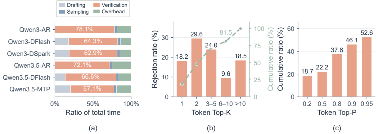
Figure 1: Execution time breakdown and rejection analysis of speculative decoding. (a) Execution time breakdown. Ratio of total time spent on drafting, verification, sampling, and overhead. (b) Target Top-K rank from rejected tokens. (c) Target Top-P distribution from rejected tokens.
