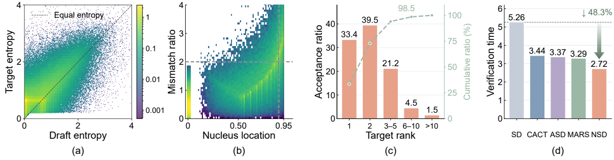
Figure 3: Nucleus-based acceptance statistics and verification efficiency. (a) Draft and target entropy. (b) Nucleus location and log probability mismatch; location zero denotes the target rank-1 token, with its strip widened for visibility. (c) Nucleus-accepted token shares and their cumulative ratio by target rank. (d) Verification time in ms/output token for Nemotron models.
