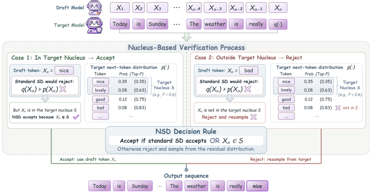
Figure 2: Overview of Nucleus Speculative Decoding (NSD).
