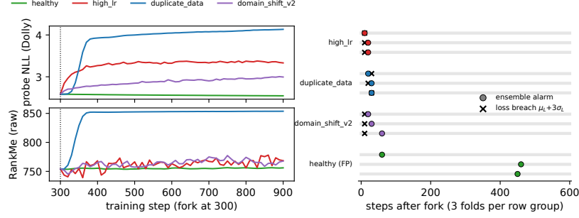
Figure 1: The negative result at a glance (Qwen3-0.6B, shared-prefix branches). Left (seed 0): duplicate_data degrades held-out NLL most while its raw RankMe rises \sim 100 above healthy — dispersion, not collapse. Right (all folds): loss breach ( \times ) and ensemble alarm ( \circ ) land within 10–60 steps of the fork and of each other — no consistent early warning — while the held-out healthy branch false-alarms at 60/460/450 steps (folds 0–2, as in Table 3).
