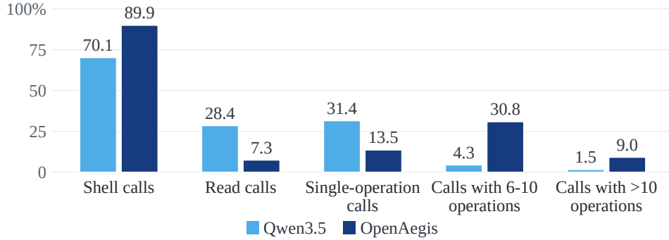
Figure 4: Tool-use and command-complexity statistics for Qwen3.5-397B-A17B and OpenAegis . Each metric is plotted independently; values are percentages of all tool calls.
