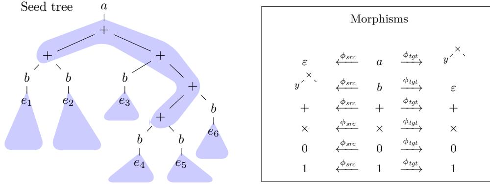
■ Figure 2 The seed tree and the morphisms generating the (source pattern, target pattern) pair capturing the transformation depicted in Figure 1.
