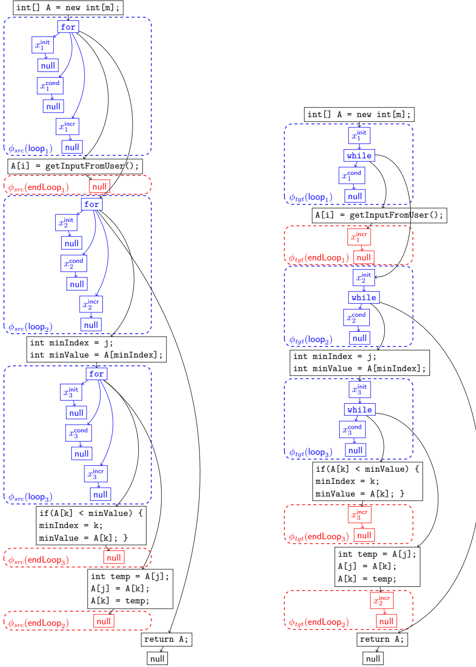
■ Figure 6 Source and target patterns. The source and target morphisms are identity everywhere, except for loop_i and endLoop_i , which are indicated by colors blue and red respectively.
