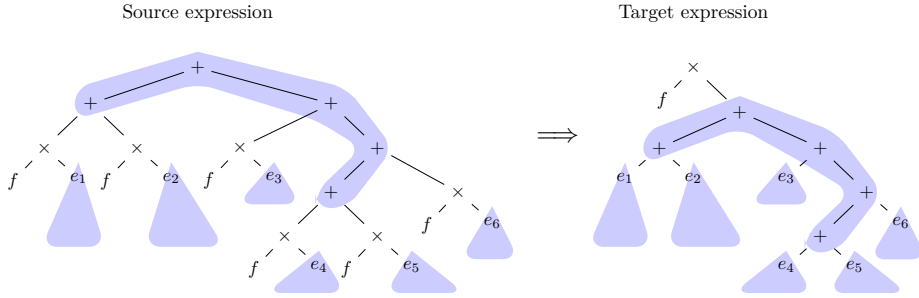
Figure 1 The transformation of an expression following distributivity. Here f, e_1, \dots, e_6 are arbitrary expressions. If f is a variable instead of an expression, we get a (source pattern, target pattern) pair that captures this transformation.
