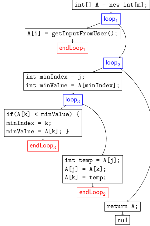
■ Figure 5 The seed tree generating the source and target patterns in Figure 6.
