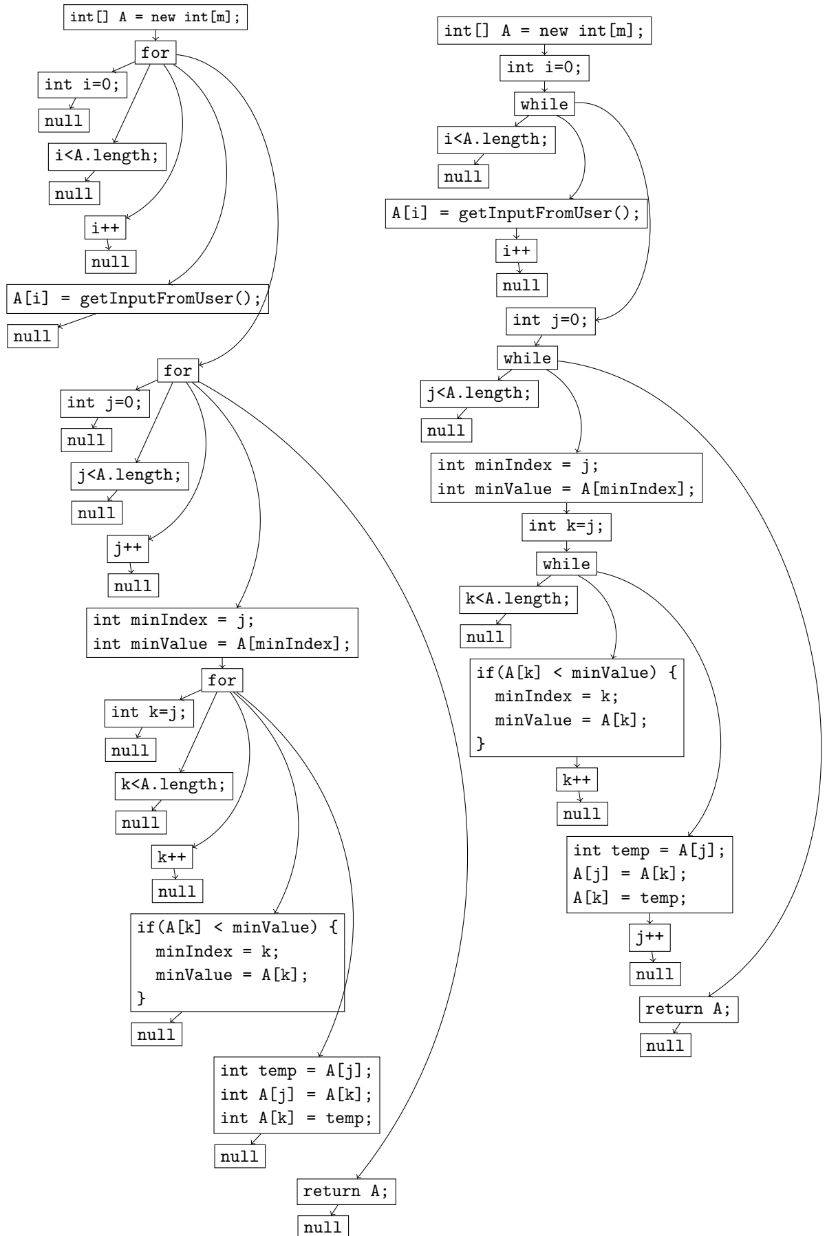
■ Figure 4 Source and target code snippets from Fig 3 as trees.
