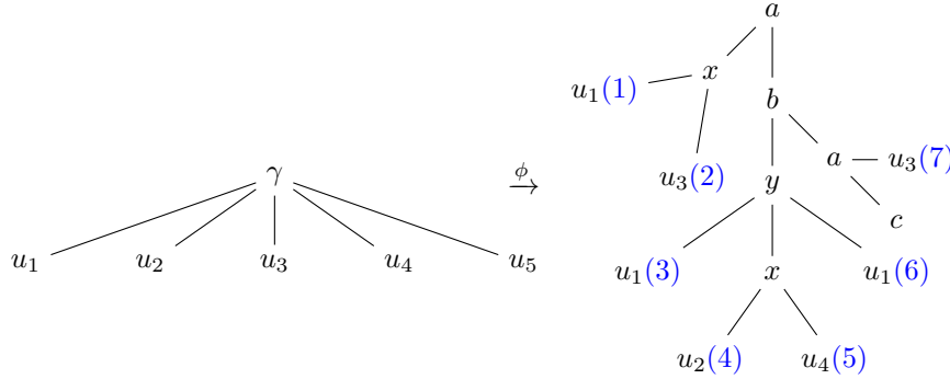
■ Figure 8 Example computation of D_\phi(\gamma)
