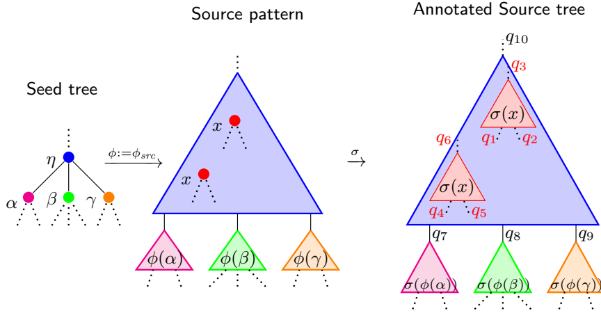
■ Figure 7 The source tree is annotated with states of \mathcal{A}_{L_{src}} . We want to simulate the effect of running \mathcal{A}_{L_{src}} on the source tree in the seed tree itself. This means, when processing \eta , it should guess and validate the potential transformation of the tuple (q_7, q_8, q_9) to q_{10} by a context (colored blue) in the source tree that matches \phi_{src}(\eta) , and simultaneously make sure that there is a substitution for x that preserves the transformations (q_1, q_2) to q_3 as well as (q_4, q_5) to q_6 . An alternating tree automaton on the seed tree can achieve this.
