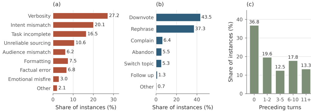
Figure 4: Composition of the experience signals: (a) failure dimension, (b) user actions, (c) preceding dialogue turns.
