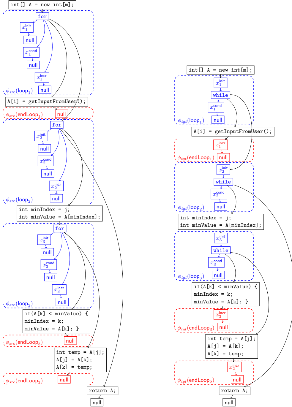
■ Figure 6 Source and target patterns. The source and target morphisms are identity everywhere, except for \text{loop}_i and \text{endLoop}_i , which are indicated by colors blue and red respectively.
