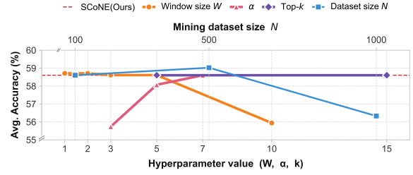
Figure 1: Ablation study on key hyperparameters using Llama-3-8B-Instruct. Results are averaged across NQ, SCIQ, and HotpotQA.
