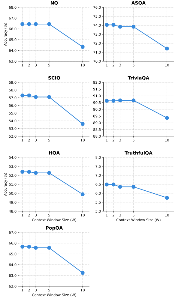
Figure 2: Performance sensitivity to context window size W .
