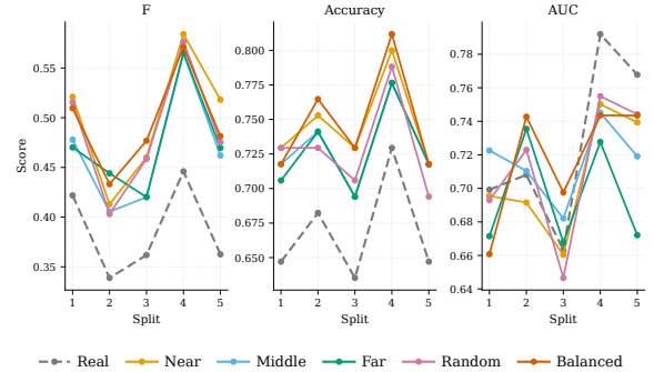
Figure 2: Split-wise performance trajectories for macro-F, accuracy, and AUC across five stratified train–test splits. Augmented conditions maintain a consistent separation above the real-only baseline (grey) for F and accuracy across all five splits. AUC shows no reliable improvement pattern. The shared performance peak at split 4 suggests this partition contains a particularly favourable distribution of boundary cases.
