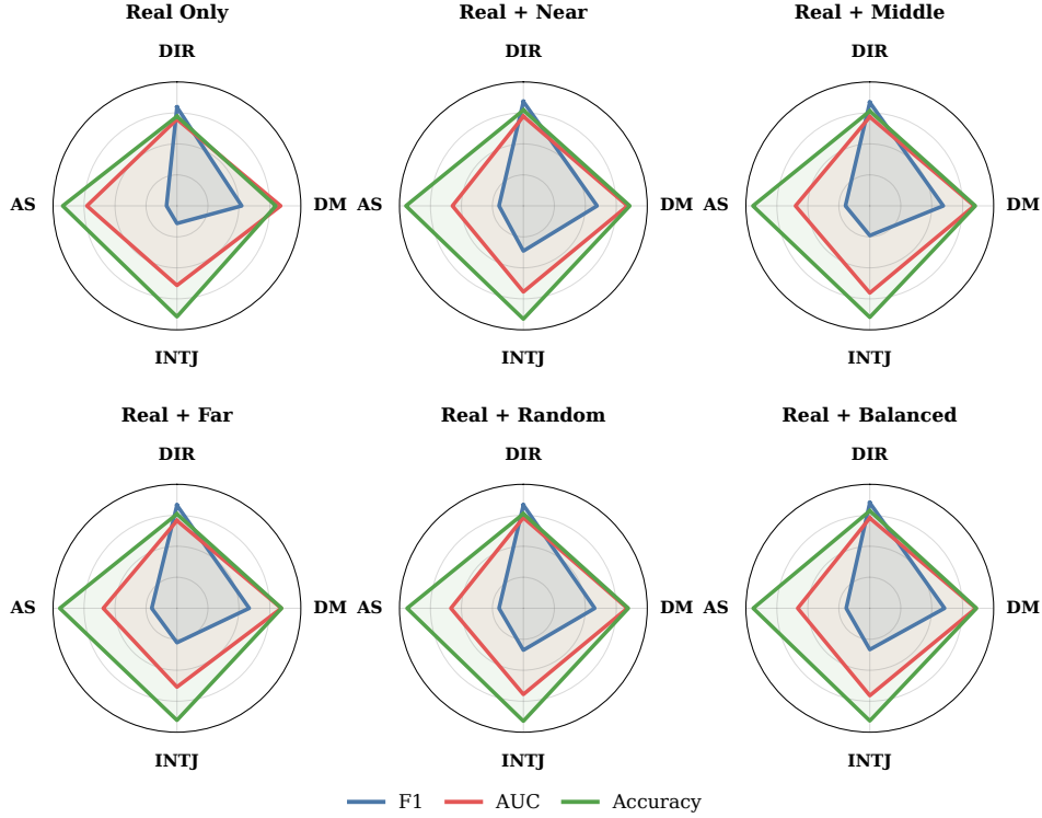
Figure 3: Per-condition radar plots showing function-level F1, AUC, and accuracy across the four discourse-pragmatic functions (DIR, AS, INTJ, DM). Each plot corresponds to one training condition. Full numeric values for all three metrics are reported in Table 12 (Appendix C). The collapsed F1 profile in the Real Only condition, particularly for INTJ, expands under augmentation, most notably under NEAR and RANDOM. AUC and accuracy profiles stay stable across conditions, consistent with the boundary-shift interpretation from Section 5.1.
