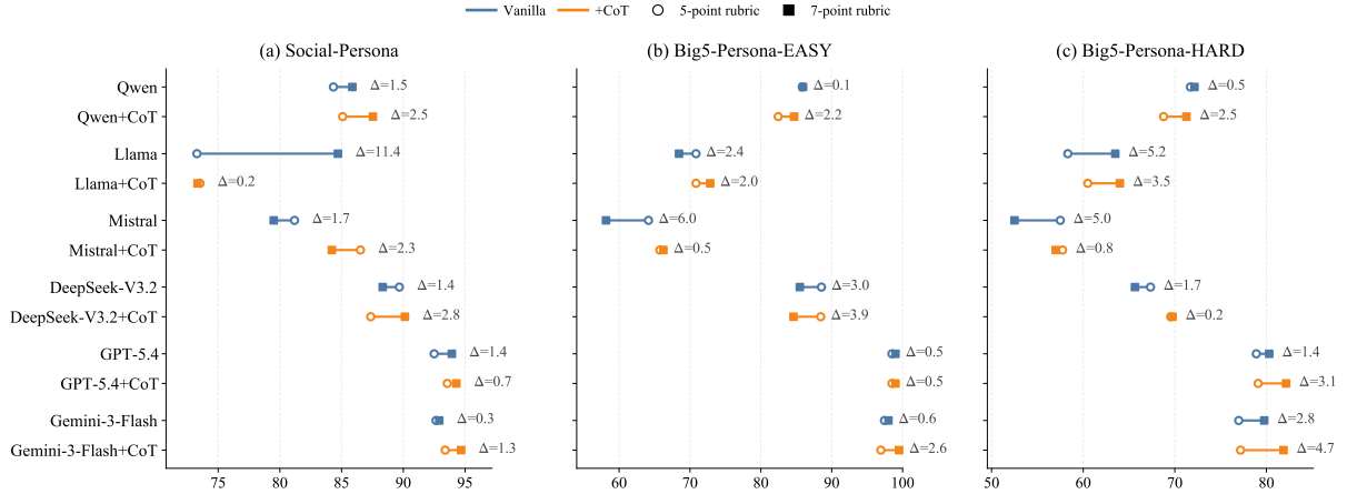
Figure 5: Rubric Sensitivity of direct LLM-as-a-Judge evaluation on Pair-AUC. Each segment connects the results from 5-point and 7-point rubrics for the same evaluator and prompting method. Longer segments indicate greater sensitivity to scoring granularity.
