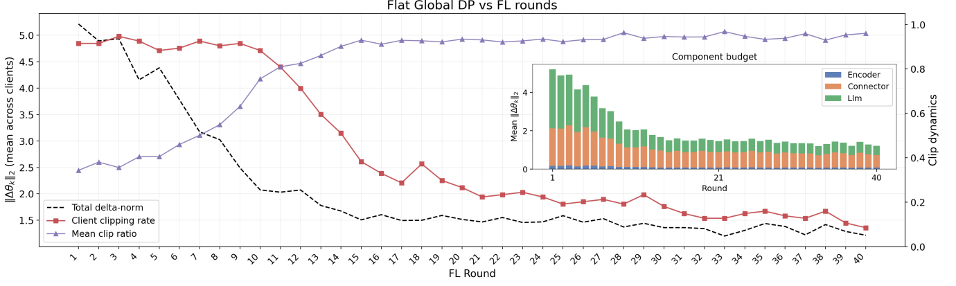
Fig. 3: Flat DP with all unfrozen components ( Flat-e baseline, 40 rounds, C=1.0 , averaging 94 clients/round). Main panel (left axis, dashed): mean total joint update norm \|\Delta\theta^{(i)}\|_2 across clients. Right axis: client clipping rate (red, fraction of clients whose update norm exceeds C ) and mean clip ratio \bar{r}^{(t)} = \frac{1}{n_t} \sum_i \min(1, C/\|\Delta\theta^{(i)}\|_2) (purple), i.e. the average fraction of each update that survives clipping before aggregation; \bar{r}^{(t)} = 1 means no client is clipped, while \bar{r}^{(t)} \ll 1 means updates are severely truncated. Inset: mean per-component norm budget per round (encoder blue, connector orange, LLM green). LLM and connector norms dominate throughout, sustaining a high global clip rate ( >80\% ) that suppresses the encoder signal to the noise floor.
