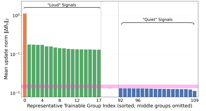
Fig. 2: Mean update norm \|\Delta\theta_h\|_2 per-Trainable Group h , i.e. LoRA matrix (log scale, sorted descending, with no-DP and all components unfrozen) for the Whisper + TinyLlama Speech-LLM. Green bars stand for LLM LoRA matrices. Blue correspond to encoder LoRA matrices. Orange (index 0) to connector (single full-rank matrix). Pink band: Gaussian noise floor \sigma C/\sqrt{n} \approx 0.01 .
