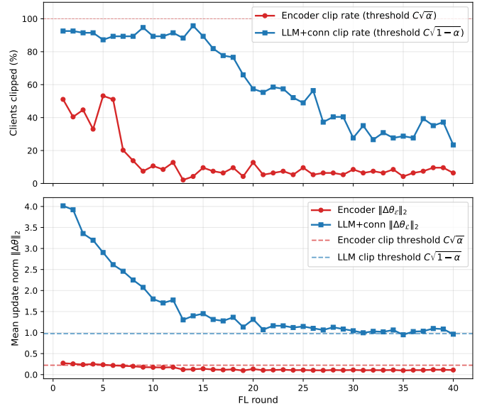
Fig. 5: Top : Per-component client clipping rate per FL round under \alpha -Split-e ( \alpha=0.05 , C=1.0 , 94 clients/round). Red: encoder pool ( C\sqrt{\alpha}=0.224 ); blue: LLM+connector pool ( C\sqrt{1-\alpha}=0.975 ). Bottom : Mean update norm \|\Delta\theta\|_2 per component—encoder \|\Delta\theta_{\mathcal{E}}\|_2 (red) and LLM+connector \|\Delta\theta_{\mathcal{L}}\|_2 (blue)—with dashed lines at the respective pool clip thresholds.
