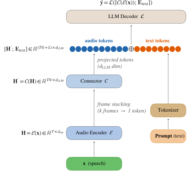
Fig. 1: Speech-LLM architecture. The audio encoder \mathcal{E} maps raw speech \mathbf{x} to frame-level representations \mathbf{H} . The connector \mathcal{C} downsamples frames, reducing sequence length by k . The LLM decoder \mathcal{L} generates the transcript \hat{\mathbf{y}} conditioned on the projected tokens and a task prompt.
