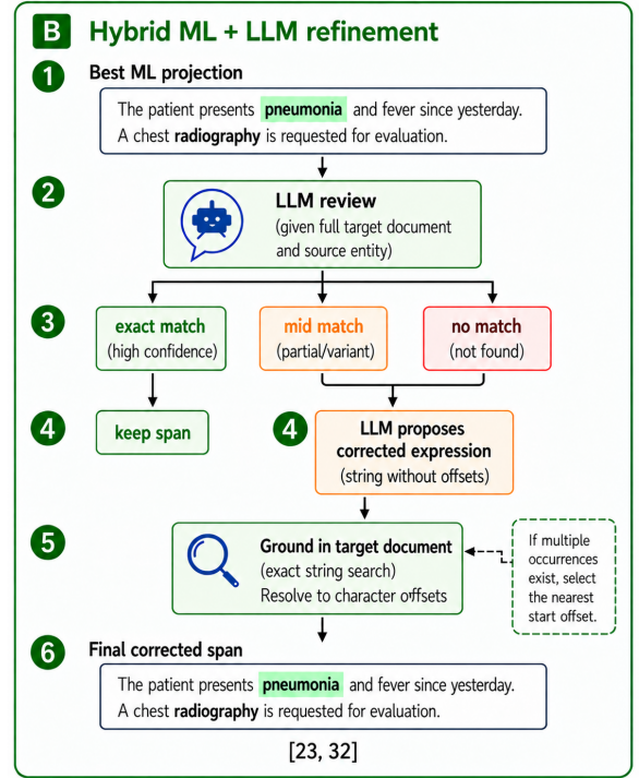
Figure 3: Overview of the hybrid ML-LLM projection approach. The best machine-learning projection is first assessed by an LLM; exact matches are retained, whereas uncertain or incorrect projections are corrected and subsequently grounded in the original target document to obtain valid character offsets.
