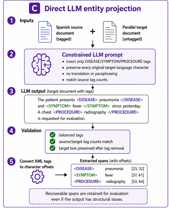
Figure 4: Overview of the direct LLM-based entity projection approach. The tagged Spanish source document and its unannotated parallel translation are provided to the LLM under constrained generation instructions. The resulting tagged target text is validated and converted into character-offset entity spans for evaluation.
