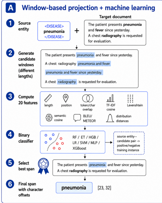
Figure 2: Overview of the window-based machine-learning approach for cross-lingual clinical entity projection. Candidate spans are generated in the target document, represented through surface, positional, structural, and semantic features, and ranked by a supervised binary classifier to select the final projected span.
