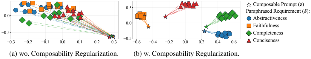
Figure 4: Qualitative visualization of projected embeddings of paraphrased requirements ( \tilde{z} ) and learned alignment-prompt representations ( z ), before and after composability regularization.
