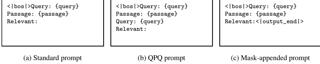
Figure 2: Prompts used for both reranker supervised fine-tuning and evaluation. (a) The standard prompt is used for Gaggle (base reranker) and all other contrastive studies by default. (b) The QPQ prompt is used for the causal query-repetition condition; both occurrences contain the same truncated query. (c) The mask-appended prompt is used for the Gaggle (MNTP) mask condition; <|output_end|> is the MNTP mask token. With the single-position readout, relevance is scored using the \text{true} minus \text{false} logits at the colon after Relevant: , immediately before the mask in (c).
