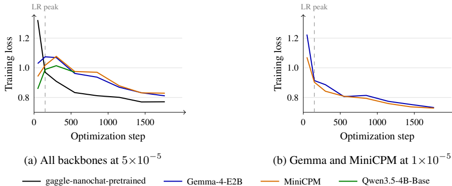
Figure 3: Training loss on identical batches at peak learning rates 5 \times 10^{-5} (a) and 1 \times 10^{-5} (b); bins widen over training to smooth per-batch noise.
