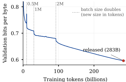
Figure 1: Validation loss on held-out ClimbMix during pre-training.
