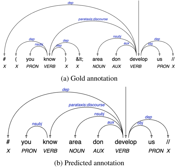
Figure 6: Gold and predicted transcription and trees for a Naija utterance (sent_id: WAZL_15_MC_AbiMG_180). The predicted annotation has all UAS, UPOS and LAS as 72.7. The scores are low because not all markups are predicted by ASR - ‘(’, ‘)’ and ‘<’ (marked as ‘&lt;’) are not predicted by ASR.
