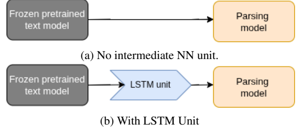
Figure 3: Text parsing with frozen text encoder - with and without intermediate NN unit.
