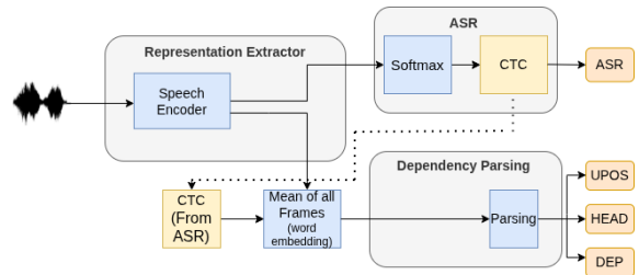
(b) Simplified Wav2tree (ours)
