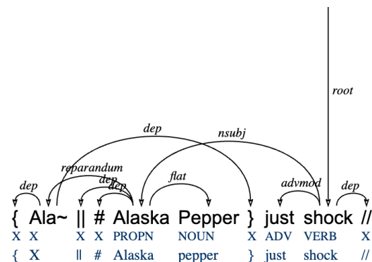
Figure 1: Dependency parsing tree from the NaijaNSC treebank. EN: Ala... Alaska Pepper was shocked. The two lines under the wordform line are the sequence of POS and lemma tags respectively.
