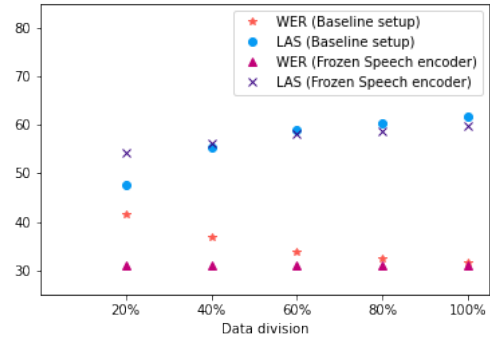
(a) Data Scaling - Naija
