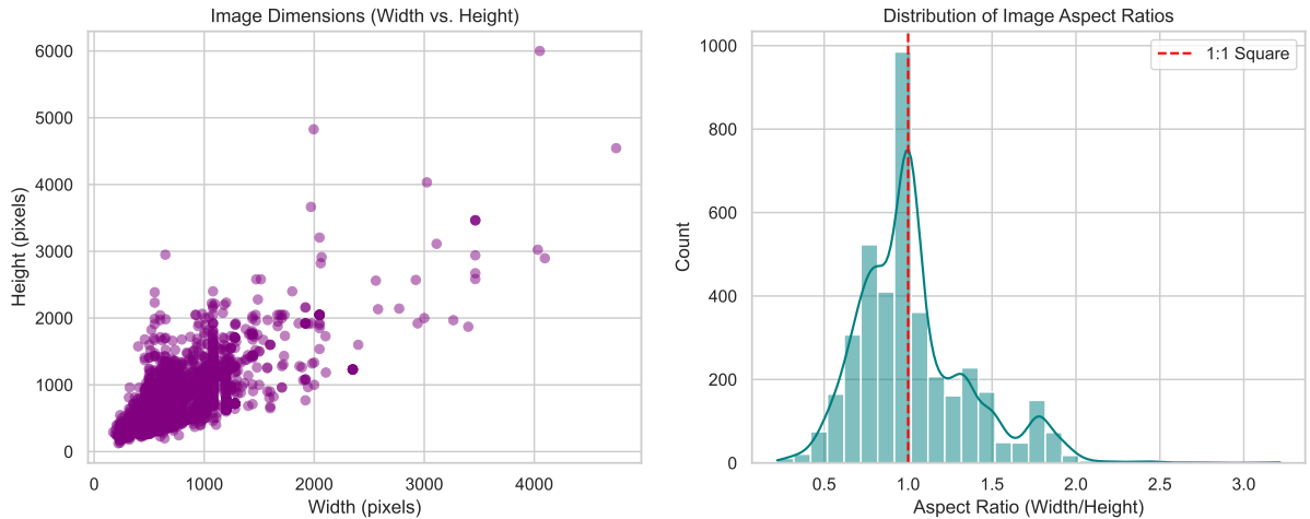
Figure 3: Image dimensions (width vs. height) and the resulting aspect ratio distribution, highlighting a dominant 1 : 1 structural format.
