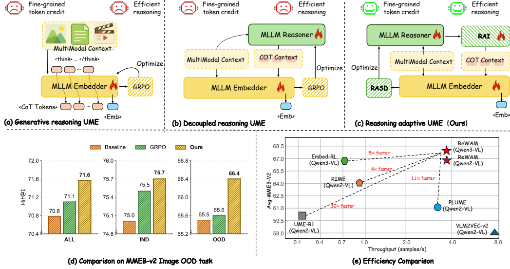
Figure 1: Overview of reasoning-enhanced UME paradigms and empirical comparisons. (a)–(c) show generative reasoning UME, decoupled reasoning UME, and ReWAM, respectively. (d) compares in-distribution and OOD retrieval, showing smaller gains from GRPO on OOD tasks. (e) compares retrieval performance and throughput across UME methods.
