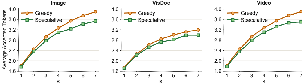
Figure 3: Ablation of retrieval-adaptive inference (RAI). Average accepted tokens as draft length K varies under greedy and speculative acceptance on MMEB-V2.
