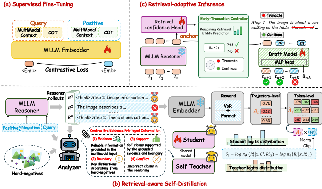
Figure 2: Overview of ReWAM. (a) Supervised fine-tuning trains a CoT-conditioned embedder. (b) RASD uses privileged same-token rescoreing to derive token-wise weights that modulate trajectory-level retrieval advantages. (c) RAI stops a partial CoT when its predicted remaining retrieval utility is low and accelerates generation through speculative decoding.
