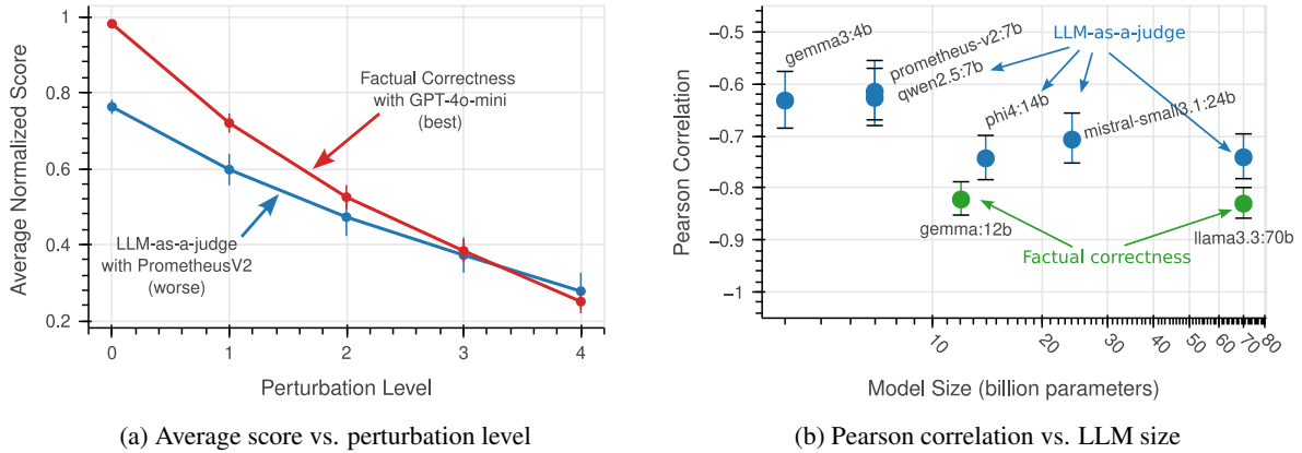
Figure 3: Performance of factuality evaluation methods.
