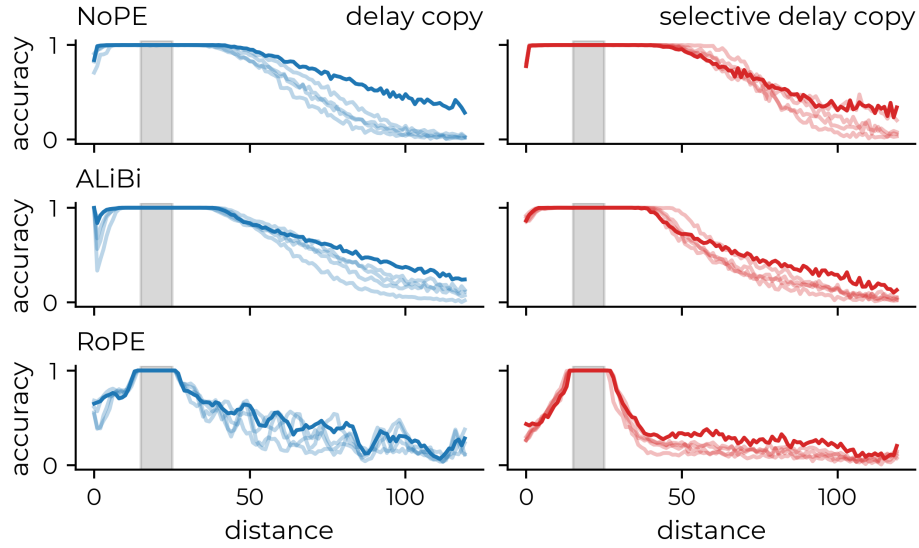
Fig. 6. For different positional encodings, we show different training runs for (left) the delay copy task ( C ), \mathcal{D}_{\text{RC}} , and (right) the selective delay copy task ( S ), \mathcal{D}_{\text{RS}} , where d_{\text{C/S}} \sim \text{unif}(15, 25) . In solid lines we show the best performing runs, measured by the integral over the full plotted distance range. These models are presented in the main text results.
