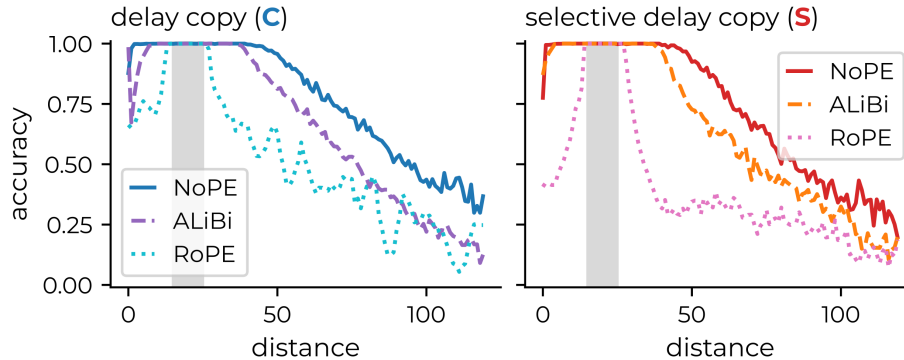
Fig. 2. Distance generalization is strongly affected by positional encoding. We compare two explicit positional encoding schemes, ALiBi and RoPE, with NoPE (no positional encoding), where NoPE relies solely on causality, viz causal attention for inferring relative distances. The evaluation accuracy is plotted as a function of the distance between source and recall, compare Fig. 1. Either all m = 10 source tokens are copied (left), the C task, or only the even component (right), denoted selective copy task S . For details see Sec. 3. During training, the model sees delay distances between 15 and 25 (gray shaded region).
