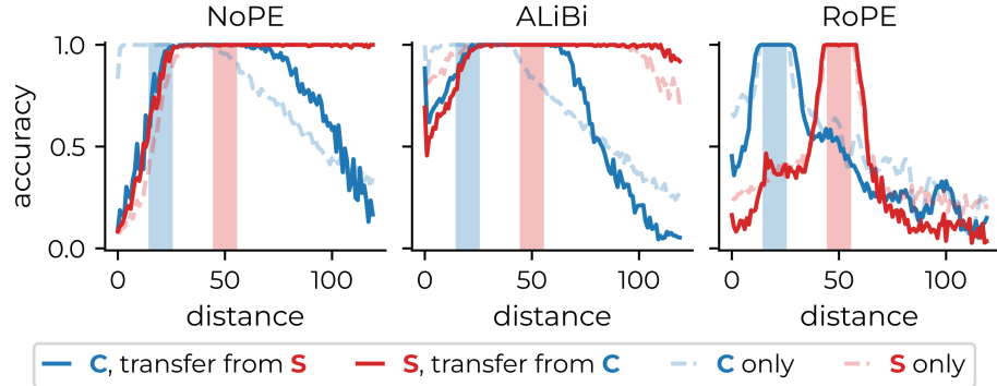
Fig. 5. Transfer learning with enlarged task separation. For three positional encoding schemes inference accuracies as a function of the source-recall distance is shown, the procedure is otherwise identical to Fig. 4. The training distances are [15, 25] for the delay copy task C , and [45, 55] for selective copy S . Solid lines are for transfer learning, when the model is trained on the joint dataset \mathcal{D}_{RCS} , dashed lines for datasets containing only one of the two tasks, either C or S .
