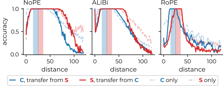
Fig. 4. Transfer learning. Shown are performance curves for three types of dataset: \mathcal{D}_{\text{RCS}} (solid lines), containing both the basic copy task (blue) and selective copy (red). Shaded regions indicate the range of the respective training delay distances. \mathcal{D}_{\text{RC}} (blue dashed), for comparison. Single task setting, here the basic copy task. \mathcal{D}_{\text{RS}} (red dashed), equivalently for selective copy.
