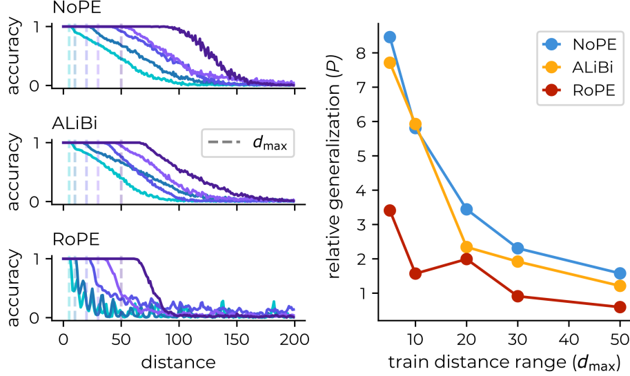
Fig. 3. Influence of data diversity on distance generalization. Shown are results for d_{\max} \in \{5, 10, 20, 30, 50\} , where distances seen during training are in [0, d_{\max}] , compare (1). Dashed lines in the left panels indicate the end of the training distance range, i.e. d_{\max} , which is taken as proxy for data diversity.
