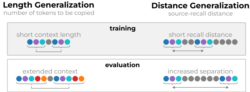
Fig. 1. Comparison of length generalization and distance generalization. Illustration for a basic copy task (see e.g. [10]). For length generalization, the model is evaluated to copy sequences longer than the training sequences, resulting in longer context lengths at inference time. For distance generalization the context length remains fixed. Instead, part of the sequence is copied with delay, where the distance between source and recall (the delay) is increased or reduced at inference time.
