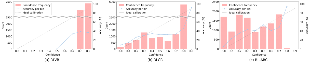
Figure 3: Performance (solid lines) and confidence frequency (bars) across confidence bins on OOD benchmarks for Qwen2.5-7B trained with each method.
