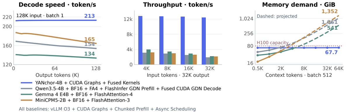
Figure 2. Single-H100 inference: sustained decoding speed, higher batched throughput, and bounded memory demand. Left: cumulative decode speed. Middle: end-to-end output throughput, selecting the batch size with the highest measured throughput for each model and input length. Right: batch-512 peak memory demand; solid curves use measured components, dashed curves project KV growth, and the dotted line marks device capacity. Appendix D gives the workloads and runtime settings.
