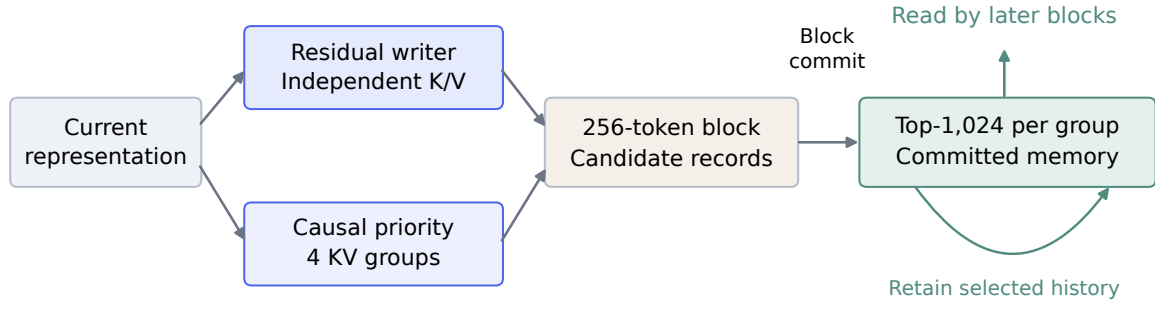
Figure 4. Causal memory maintenance. An independent writer produces K/V representations, and a causal network supplies group-specific admission scores. Each 256-token block selects a persistent Top-1,024 set per KV group. Retained records preserve their written representations as memory anchors for subsequent retrieval.
