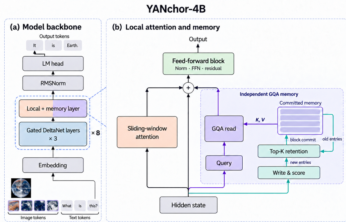
Figure 3. Architecture of YANchor-4B. Recurrent layers are interleaved with local-attention and memory modules. The inset shows how explicit records are written, retained as memory anchors, and retrieved through an independent read path. All history paths have fixed capacity. Image credit: NASA.
