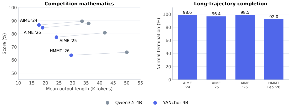
Figure 6. Competition performance and generation behavior. Left: benchmark score against mean output length; each line connects YANchor and Qwen3.5-4B on the same benchmark. Right: YANchor’s normal-termination rate across the four competition sets. Accuracy measures successful solutions; normal termination measures reaching EOS before a stopping limit.
