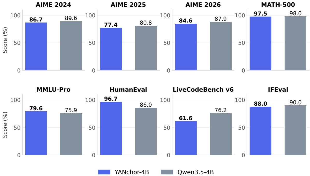
Figure 7. Cross-architecture comparison of YANchor-4B with the original Qwen3.5-4B, a Gated DeltaNet/global-attention hybrid, across mathematics, knowledge, code, and instruction following. Scores use the primary metrics defined in Section 5.
