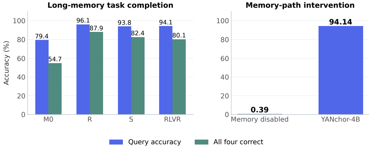
Figure 8. Long-memory task accuracy. Left: M0, R, S, and RLVR. Right: the released model with memory disabled or enabled.
