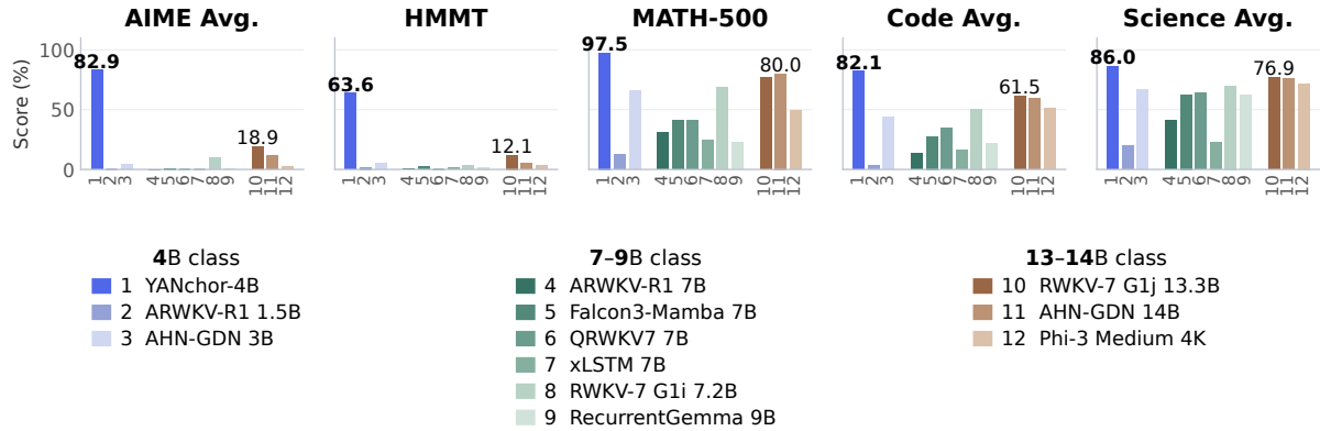
Figure 1. YANchor-4B and 11 bounded-state baselines on mathematics, code, and science. Models are grouped by parameter scale. Avg. denotes an equal-weight benchmark mean: AIME covers 2024–2026; Code covers HumanEval, MBPP, and LiveCodeBench v6; Science covers GPQA-Diamond, ARC-C, and ARC-E. HMMT uses February 2026. Section 5 defines the primary metrics.
