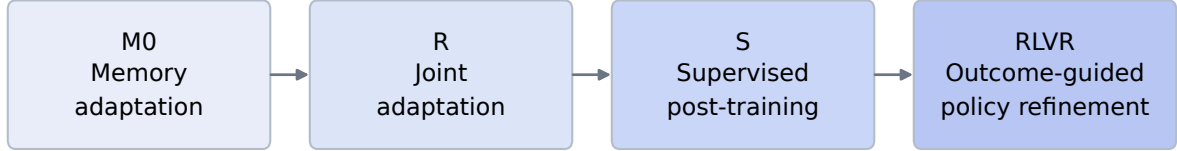
Figure 5. The M0, R, S, and RLVR training sequence for YANchor-4B.
