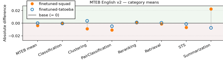
Figure 5: Performance on the MTEB benchmark categories for fine-tuned models. The absolute differences are small, meaning our fine-tuning setup does not affect the overall performance.
