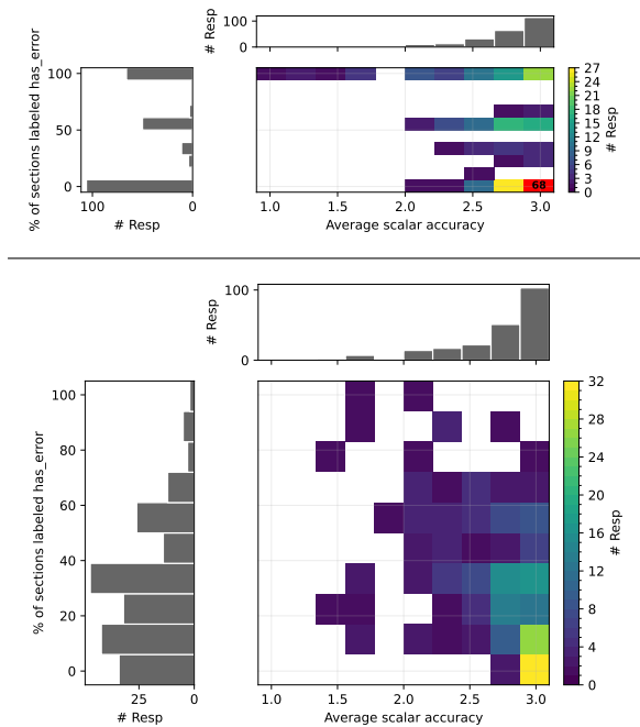
Figure 2: Relationship between average response-level accuracy and the percentage of sections labeled has_error for responses with 1–2 sections (top, 241 responses) and 3+ sections (bottom, 217 responses). Marginal histograms show the response-count distributions along each axis: % of sections labeled has_error on the y-axis and average response-level accuracy on the x-axis. Color indicates the number of responses at each point; white cells indicate unobserved combinations. In the top panel, the red cell exceeds the displayed color scale and is labeled with its exact count (68).
