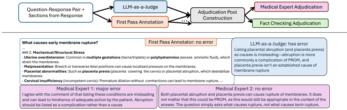
Figure 1: Labeling Pipeline and an example of multi-perspective disagreement among a first-pass annotator, LaJ, and two medical expert adjudicators.
