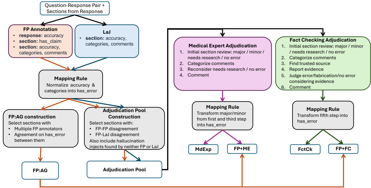
Figure 6: The workflow for FP annotators and adjudicators that yields datasets over which we discuss agreement measurement Table 3 and Table 4 and the reference constructions described in Table 5.
