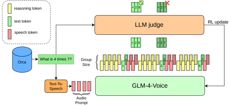
Figure 1: Illustration of our RL pipeline. We synthesize as speech a question taken from the Orca dataset (Mitra et al., 2024) to be fed to the GLM-4-Voice (Zeng et al., 2024), and generate multiple interleaved speech-text replies. We apply a group-relative policy-gradient objective inspired by GRPO (Shao et al., 2024), using a binary reward obtained from a large language model applied to the decoded text stream. The model can optionally use interleaved reasoning tokens following Chiang et al. (2026).
