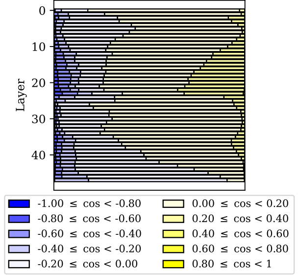
Figure 22: Distribution of neurons by layer and input-output weight cosines in T5-large models (visualization of Table 6). Layers 0-23 correspond to the encoder, and 24-47 to the decoder.
