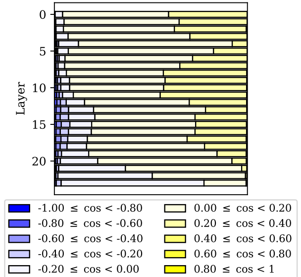
Figure 23: Distribution of neurons by layer and input-output weight cosines in BERT-large-cased (visualization of Table 7).
