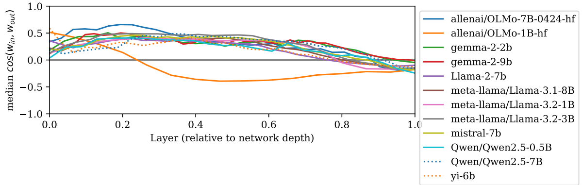
Figure 26: Median of \cos(w_{in}, w_{out}) by layer (x-axis) for all 12 models investigated. Unlike Fig. 2 we also include the models of 1B parameters and below. All models follow the same general pattern, but OLMo-1B switches to negative values earlier than the others.
