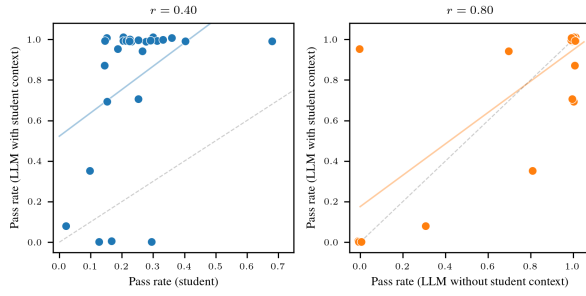
Figure 20: Problem-level pass rate correlations for Opus 4.6 on DSA HK231. Left: student pass rate vs. LLM pass rate with student context ( r = 0.40 ). Right: LLM pass rate without student context vs. LLM pass rate with student context ( r = 0.80 ). The stronger correlation between the two LLM conditions suggests the LLM’s performance on each problem is driven primarily by its own coding ability rather than the student profile.
