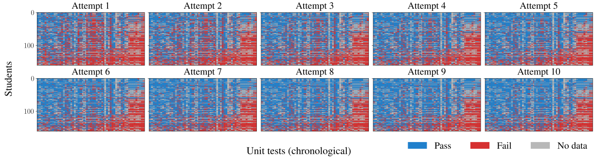
Figure 4: Per-attempt correctness heatmap of students on DSA HK231. Each of the ten panels shows one attempt number. Within each panel, the vertical axis is students (one row per student, sorted by overall pass rate) and the horizontal axis is test cases (one column per test case, ordered chronologically); blue marks a passed test case and red a failed one. The progressive expansion of blue from attempt 1 to attempt 10 shows students mastering additional test cases through repeated practice.
