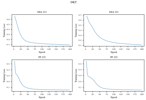
Figure 15: DKT training loss across 200 epochs. The LSTM converges more slowly than the parametric models.
