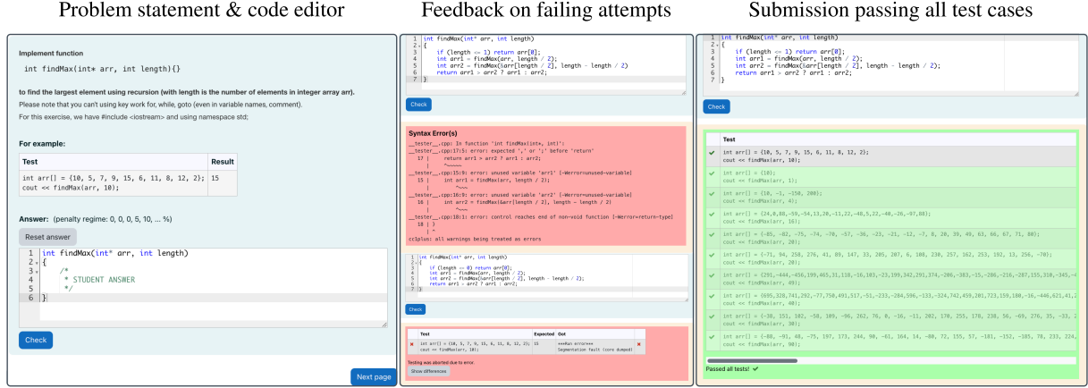
Figure 1: The exercise platform interface based on Moodle. From left to right: the problem statement with function signature, description, example test case, and the code editor where the solution attempt is written; automated feedback on failing attempts, with compiler errors (red) and failed test cases showing expected versus actual output; and a revised submission where all test cases pass (green).
