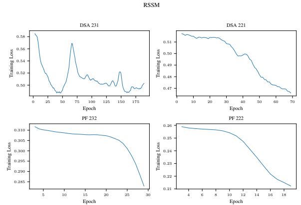
Figure 19: RSSM training loss across epochs for all four course offerings, plotted up to the checkpoint selected by validation AUC.
