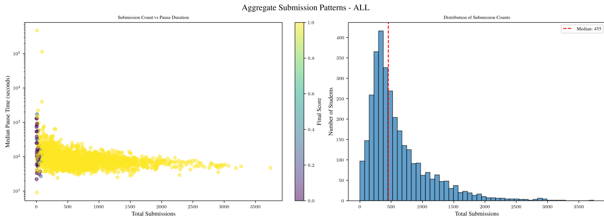
Figure 10: Aggregate submission pacing patterns across all students and courses. (Left) Scatter plot of total submissions vs. median pause time, colored by final score. (Right) Distribution of total submissions per student, with the median (455) marked by the dashed red line.
