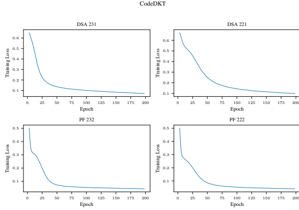
Figure 16: Code-DKT training loss across epochs for all four course offerings.
