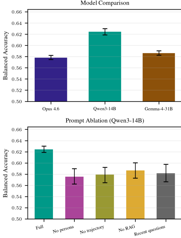
Figure 6: LLM predictor analysis on DSA HK231. Top: model comparison. Qwen3-14B achieves the highest balanced accuracy, outperforming Gemma-4-31B and Opus. Bottom: prompt ablation on Qwen3-14B. The full prompt outperforms all ablated variants.
