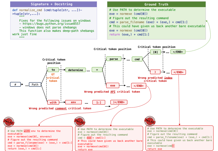
Fig. 2. Motivating example from CoderEval task 62e4fb4d [7]: critical tokens exhibit diverse syntax and can appear in multiple roles ( normalize_cmd scenario).
