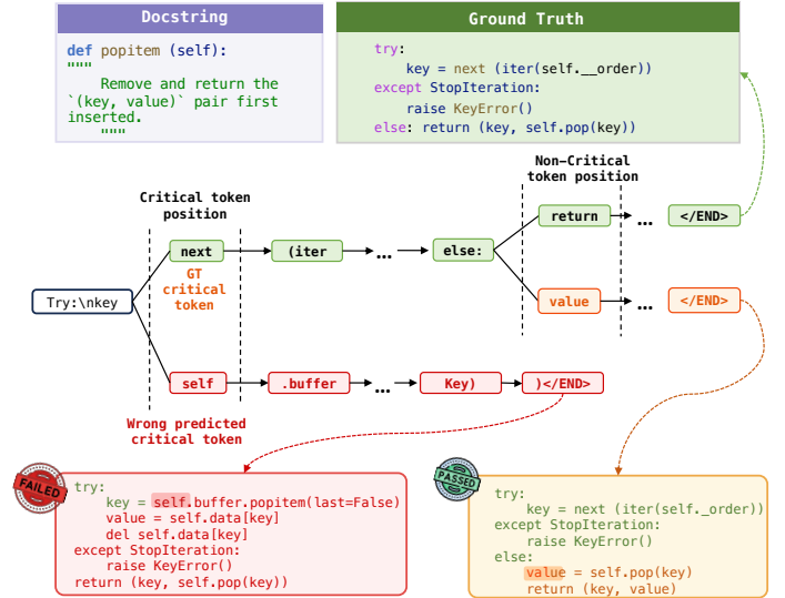
Fig. 1. Motivating example from CoderEval task 62b8d22f [7]: an incorrect critical token can cause catastrophic failure in subsequent generations ( popitem scenario).
