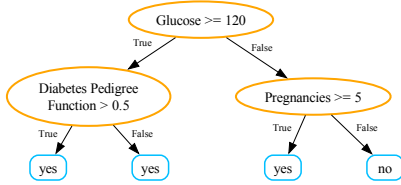
Figure 15: An Example of GPTree
