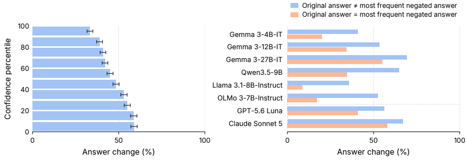
Figure 2: Left: Answer change rates decrease with confidence in the original answer (mean token log-probability; results averaged across six open-source models). Right: Answer change rates are also lower when the original answer is the model’s most common response under negation.
