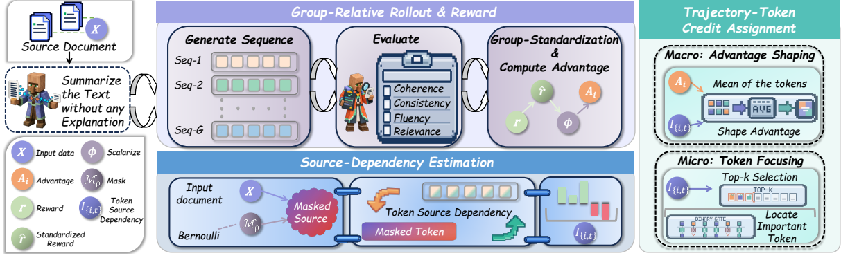
Fig. 2. The logic implementation of our proposed TIAO.
