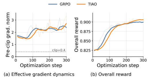
Fig. 3. Case study on effective gradient dynamics and overall reward. (0.960), the highest consistency (0.946), and a much lower STD. This indicates that moderate perturbation provides more balanced source-dependency signals than too weak or too aggressive masking.
