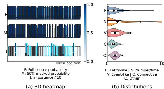
Fig. 1. TIAO token dependency analysis under source masking. (a) compares full-source and masked-source token probabilities and highlights source-dependent update positions. (b) summarizes trajectory-level dependency patterns across token categories.
