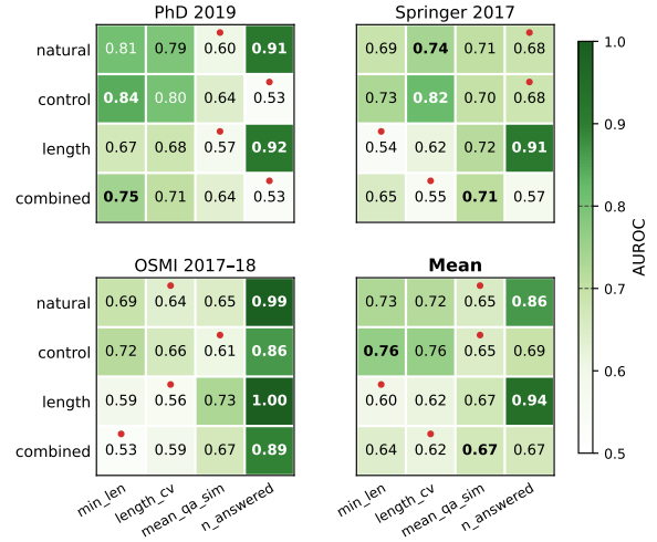
Figure 1: Cue AUROC across four prompting modes (natural, controlled, length-restrictive, combined) and three surveys. Rows: prompting modes; columns: cues.
