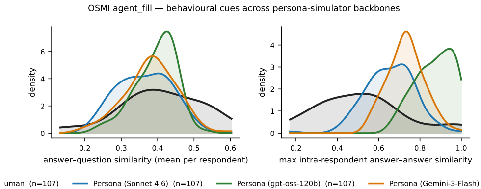
Figure 4: Cross-LLM behavioural cues on osmi_mh: mean_qa_sim (left) and max_aa_sim (right) KDEs for human respondents and three persona-simulator backbones (Sonnet, gpt-oss-120b, Gemini-3-Flash). Sonnet and Gemini sit just to the right of the human distribution on mean_qa_sim , supporting the LLM-family-independent on-topic-ness cue; gpt-oss-120b exhibits a sharp max_aa_sim shift due to intra-respondent answer reuse.
