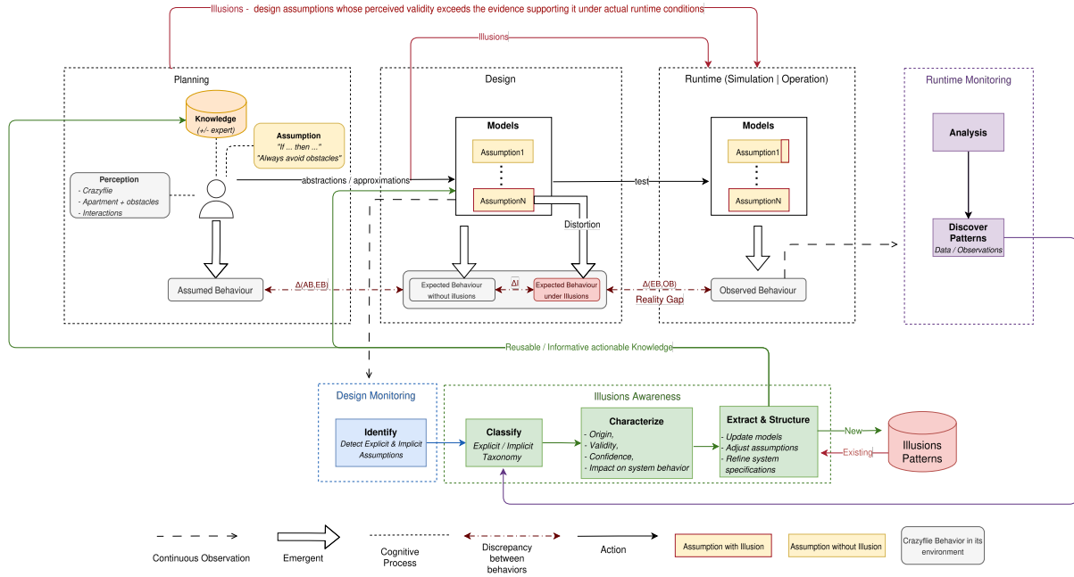
Figure 2: A Conceptual Pipeline for Design Illusions Awareness
