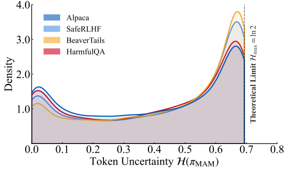
(a) Uncertainty distribution across domains.
