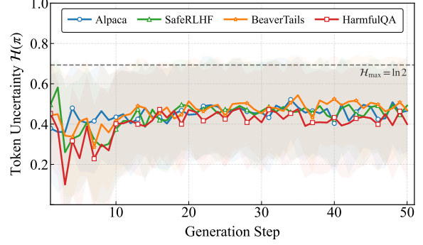
(b) Uncertainty over generation steps.
