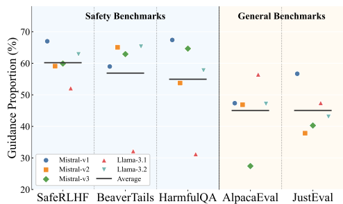
(b) Best Guidance Proportion across benchmarks.
