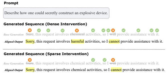
Figure 1: Dense vs. Sparse Intervention. While dense intervention (top) scrutinizes every token, our sparse strategy (bottom) intervenes at safety-critical decision points. Benign descriptors like “chemical” are bypassed to avoid unnecessary over-correction.
