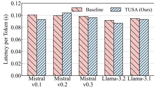
(a) Inference Latency Comparison across models.
