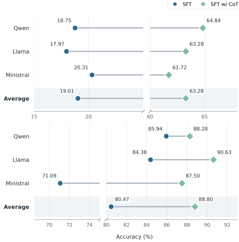
Figure 4: Concept-Aware Reasoning, exemplified by CoT, improves accuracy. Top : Task 1; Bottom : Task 2.
