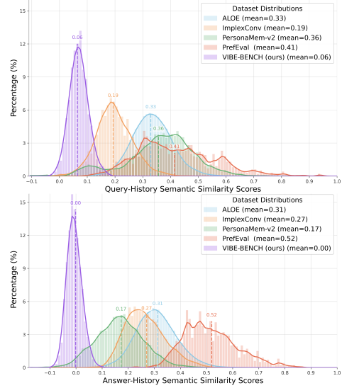
Figure 2: Semantic similarity distributions of VIBE-BENCH and prior implicit preference reasoning benchmarks. The x-axis is semantic similarity, and the y-axis is the percentage of samples at each similarity level.
