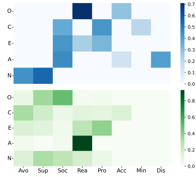
Figure 5: Big Five-emotion-regulation strategy mappings. Blue : dataset ground-truth distribution; Green : zero-shot induced distribution by GPT-5-mini.
