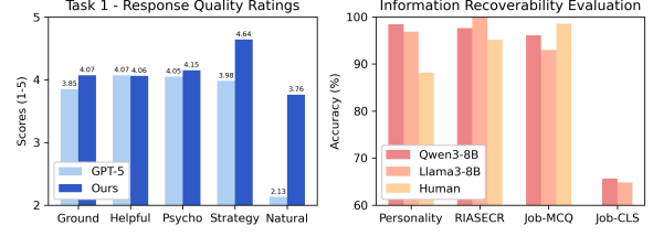
Figure 3: Dataset Quality Assessment. Left : Five-dimensional evaluation of Task 1 generation quality. Right : Recovery of profile information from dialogue histories. Job-MCQ uses four sampled distractor occupations, while Job-CLS is candidate-free.
