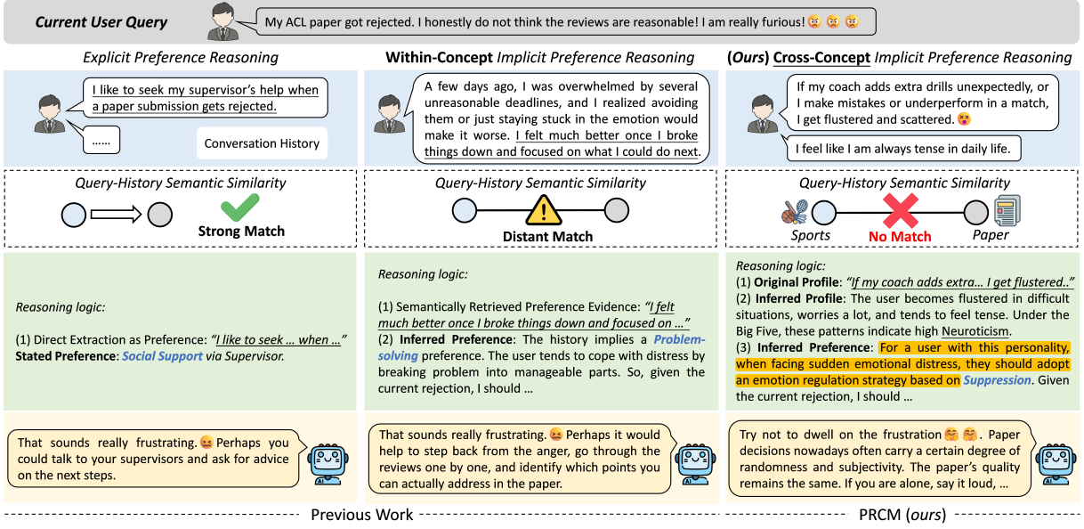
Figure 1: Illustration of three preference-reasoning regimes in PLLMs. In cross-concept implicit preference reasoning (our focus, PRCM), observable profile cues and target preferences lie in different concept spaces, requiring inference through cross-concept mappings rather than the direct semantic matching assumed in previous work.
