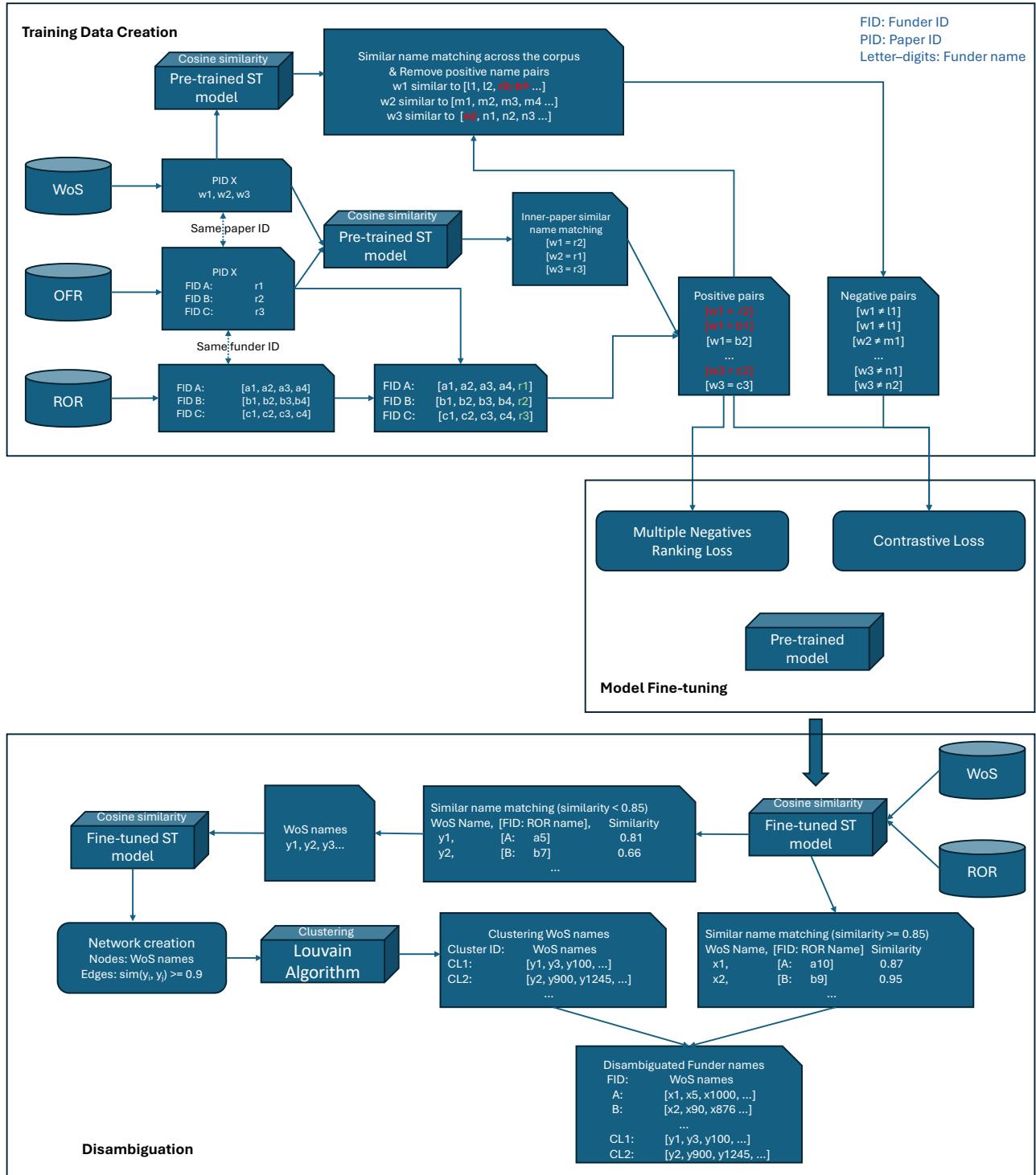
Figure 3. Steps for training data creation, model fine-tuning, and funder name disambiguation. Paper refers to a published research article. Funder name refers to a single textual representation of a funding organization as it appears in a paper. Funder ID refers to the unique identifier assigned to a funder. Multiple funder names across different papers may refer to a single funder. Therefore, we use the funder ID to link these name variants to the same underlying entity.
