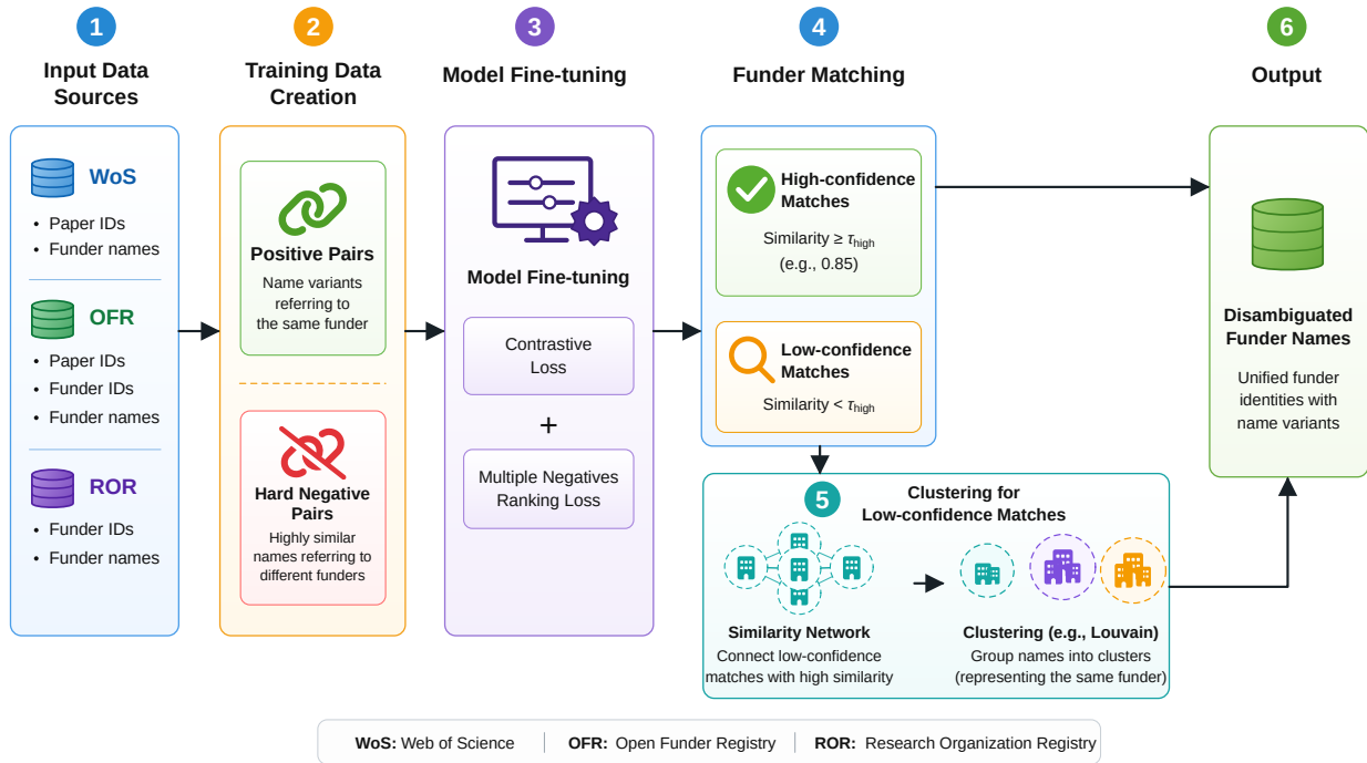
Figure 1. Overall funder name disambiguation workflow
