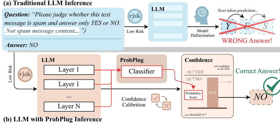
Fig. 1. Motivation for the proposed method. (a) Traditional LLM inference relies on next-token probabilities, which are often poorly calibrated and difficult to threshold in high-stakes settings. (b) ProbPlug estimates confidence from multi-layer hidden representations of a frozen LLM, enabling reliable and flexible threshold-based filtering.
