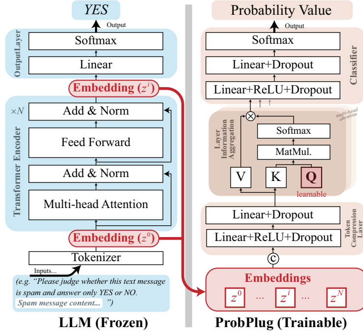
Fig. 2. The overview of the proposed method. The left sub-figure illustrates the frozen large language model, while the right subfigure presents the architecture of our proposed ProbPlug.
