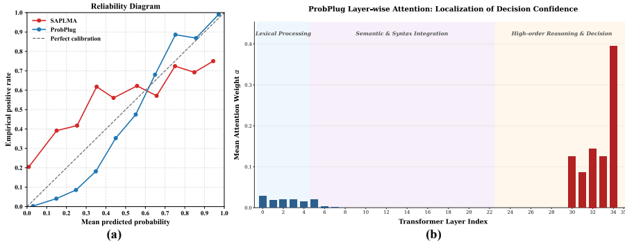
Fig. 3. (a)Reliability diagrams of confidence calibration for SAPLMA and ProbPlug on Amazon-polarity. (b)Visualization of the learned attention weights \alpha across the 36-layer base model. The distribution demonstrates the concentration of decision certainty within the terminal high-order reasoning layers (L30L35).
