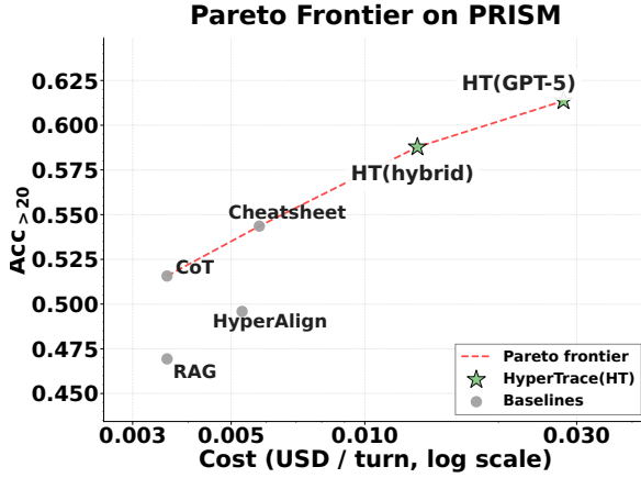
Figure 6: Cost–accuracy trade-off on PRISM, measured by online cost per turn and \text{Acc}_{>20} . HT(gpt-5) gives the strongest accuracy, while HT(hybrid) provides a more practical Pareto point.
