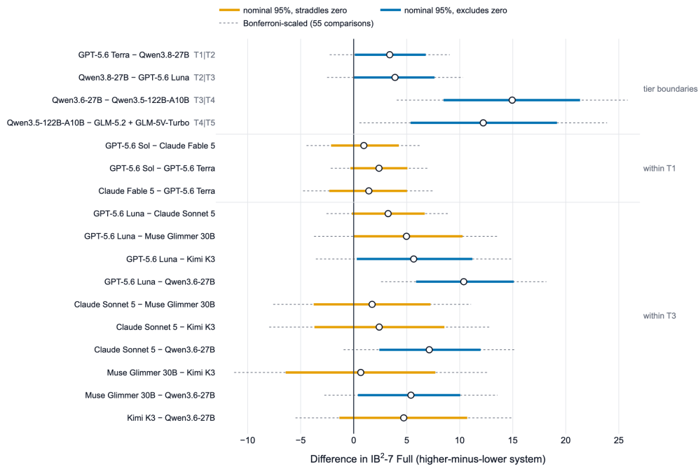
Figure 4: The intervals the nominal tier construction rests on: the four tier-boundary cuts, all three within-T1 pairs, and all ten within-T3 pairs, each stated as higher-minus-lower so no sign convention is needed. Solid bars are the released 95% percentile intervals of Algorithm 4, blue where they exclude zero and orange where they straddle it; the open marker is the observed difference. The dotted bar is a Bonferroni-scaled band at \alpha/55 . It is a normal-approximation rescaling of the released interval, not a recomputed adjusted percentile interval, because the 20,000 retained draws are held in the sealed run evidence rather than in pairwise_intervals.csv ; it is a display of the multiplicity argument in Section 6.1, not a second inferential claim. Both top cuts lose zero exclusion under it while both lower cuts keep it, which is the T1–T3 merge that paragraph describes.
