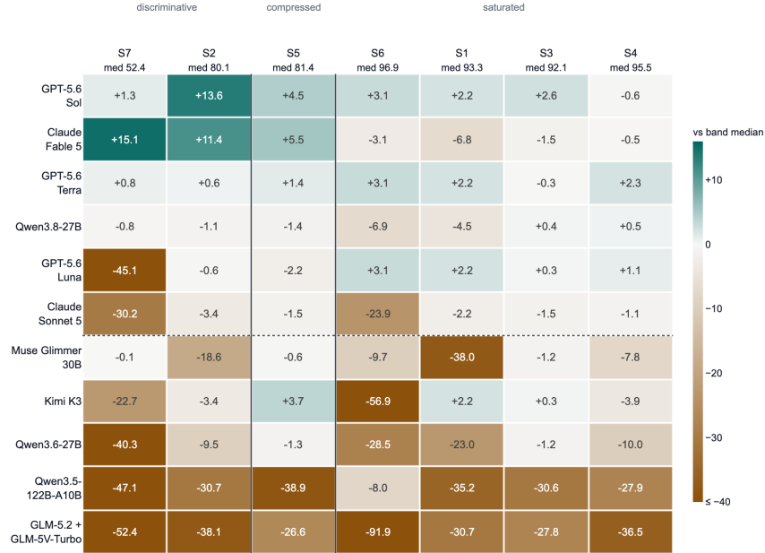
Figure 2: Suite profiles as deviation from the top-six band median , which is the quantity Definition 2 classifies on and the one Table 8 cannot show at a glance; each column header carries its band median, so any cell’s raw score is the header plus the printed deviation. Systems are ordered by IB 2 -7 Full and columns follow Table 8’s ordering rule exactly. Vertical rules separate the discriminative suites (S7/S2), the compressed-below-ceiling suite (S5), and the four saturated suites; the dotted horizontal rule marks the bottom of the six-system band the medians are computed over. The four right-hand columns are near-white across the band, which is what “nearly uniform at the frontier” means, while S7 and S6 carry deviations of tens of points for systems that are otherwise close. Colour saturates at \pm 40 so that one cell does not set the scale for all 77; six cells exceed it, and every cell prints its own exact deviation regardless.
