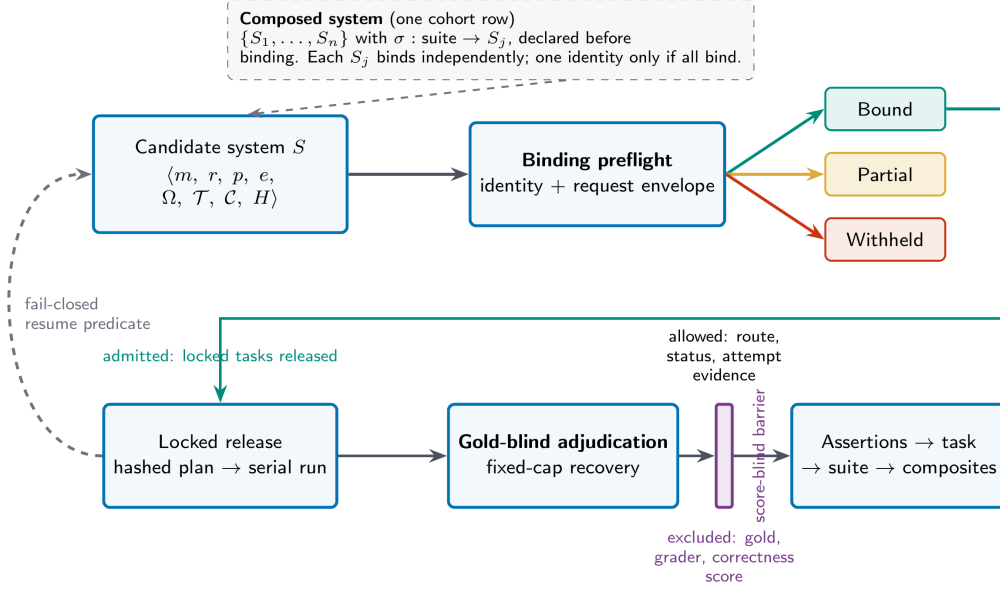
Figure 1: The IB 2 protocol. Binding has three explicit dispositions before a locked task is released. Adjudication receives only the allowlisted projection; gold, grader output, and correctness scores remain outside the recovery selector. The dashed edge is the fail-closed resume predicate.
