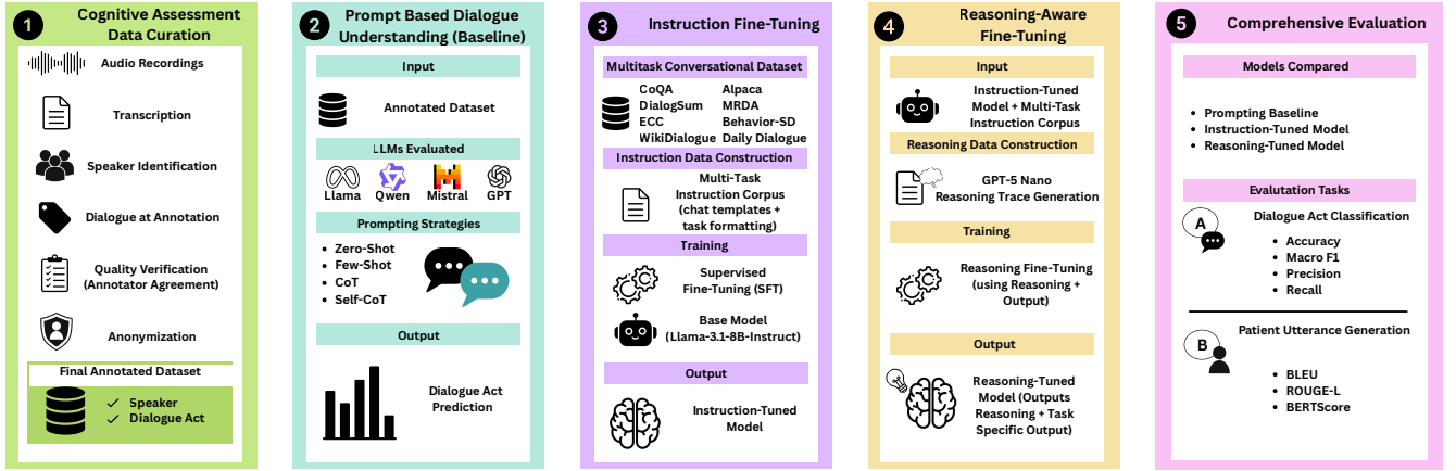
Figure 1: Overview of the data construction, model adaptation, and evaluation tasks.
