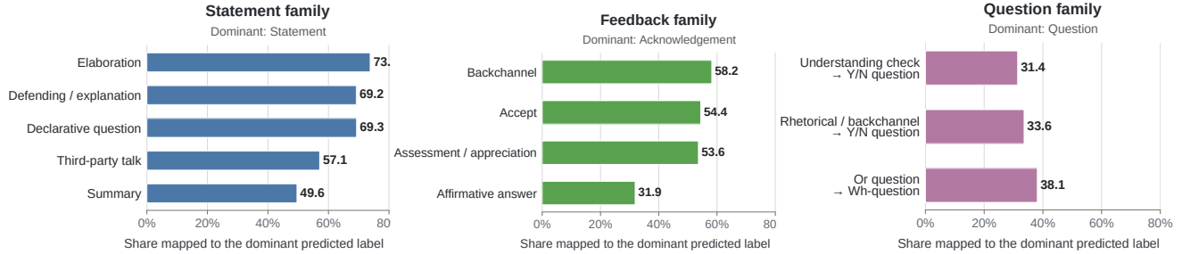
Figure 2: Dominant prediction patterns within each dialogue-act family. Each bar shows the percentage of examples mapped to the family’s dominant predicted label.
