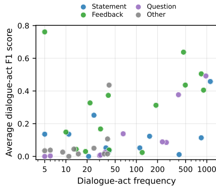
Figure 3: Dialogue-act frequency versus average F1, grouped by dialogue-act family.
