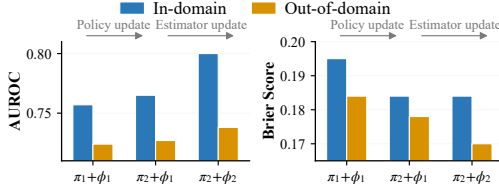
Figure 3: Step-wise effects of IPoET, showing that both policy and estimator updates progressively improve confidence estimation.
