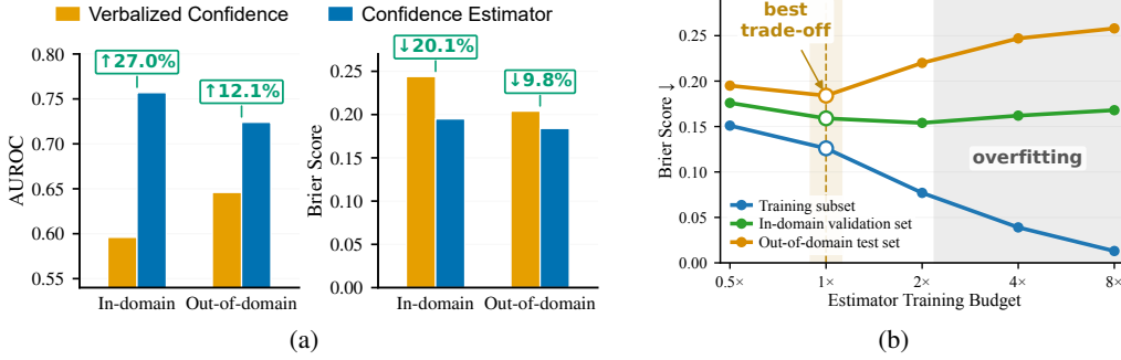
Figure 1: (a) In-domain and out-of-domain comparison of confidence estimator and verbalized confidence using AUROC and Brier score. Percentages denote relative improvements over verbalized confidence. (b) Estimator performance across training budgets: Brier scores on a training subset, an in-domain validation set, and an out-of-domain test set illustrate overfitting with extended training.
