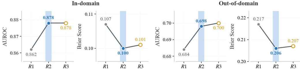
Figure 4: Round-wise comparison of in-domain and out-of-domain AUROC and Brier score under Big-Math training. Blue shading marks the configuration used in our main experiments (Round 2).
