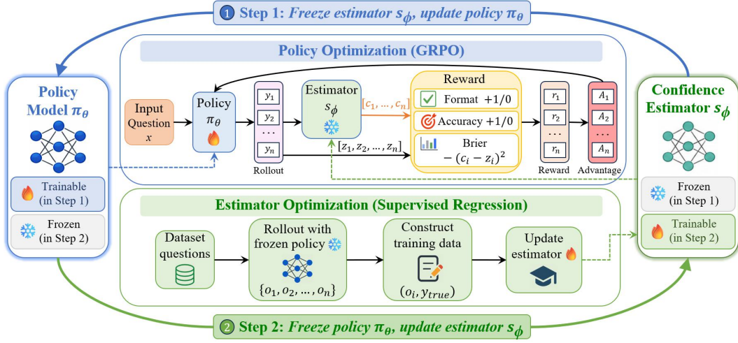
Figure 2: Overview of IPoET. The framework alternates between policy and estimator optimization. In the policy-update stage , the confidence estimator is frozen and provides confidence estimates to form an estimator-derived term, combined with format and accuracy rewards for GRPO. In the estimator-update stage , the policy is frozen to generate correctness-labeled rollouts for updating the estimator via supervised regression. Across iterations, the policy refines reasoning-oriented generation while the estimator adapts to the evolving policy distribution.
