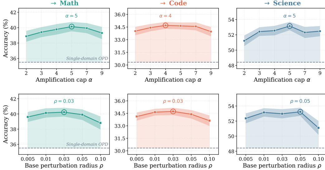
Figure 5: Sweeps over the two hyperparameters of USA on the Qwen3-1.7B students. The top row varies the amplification cap \alpha of Eq. (9) and the bottom row varies the base radius \rho of Eq. (10), each with the other held at its default. Each column fixes a target domain and each point averages the two transfer directions of Table 1 that share it, so either row covers the six directions once. The band is the standard deviation over five runs, the dashed line is the Single-domain OPD reference of Table 1, and the circled marker is the peak of that curve.
