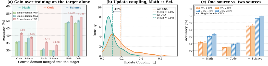
Figure 3: Where the gain of USA comes from, and what happens when a second source is added. (a) Each transfer direction under three training configurations, separating the gain of update-aware training on the target from that of merging a source. (b) Per-parameter update coupling |c_i| of Figure 1(d) on Math \leftrightarrow Science, for experts trained by plain OPD and by USA. (c) Both remaining domains merged into the target, against the single-source results of Table 1; Appendix G.1 examines more. Error bars in (a) and (c) are standard deviations over five runs.
