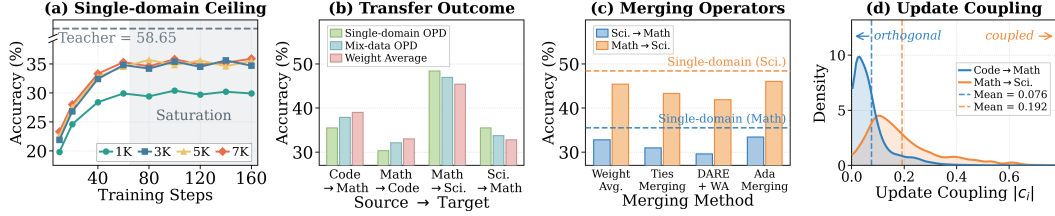
Figure 1: Motivation and diagnosis of cross-domain OPD via model merging. (a) OPD on Math saturates early, and scaling the corpus from 1K to 7K cannot break the ceiling. (b) Gains polarize across domain pairs: Code \leftrightarrow Math improves in both directions, Math \leftrightarrow Science degrades in both. (c) On the conflicting pair, all four merging operators fall below the single-domain baseline. (d) Per-parameter update coupling |c_i| = 2|\Delta_t(i)\Delta_s(i)|/(\Delta_t(i)^2 + \Delta_s(i)^2) with \Delta_k = \theta_k - \theta_0 , being 0 when only one domain updates it and 1 when both do comparably. The facilitating pair concentrates near 0, the conflicting pair shifts right. Appendix C.6 explains why it ignores the two signs.
