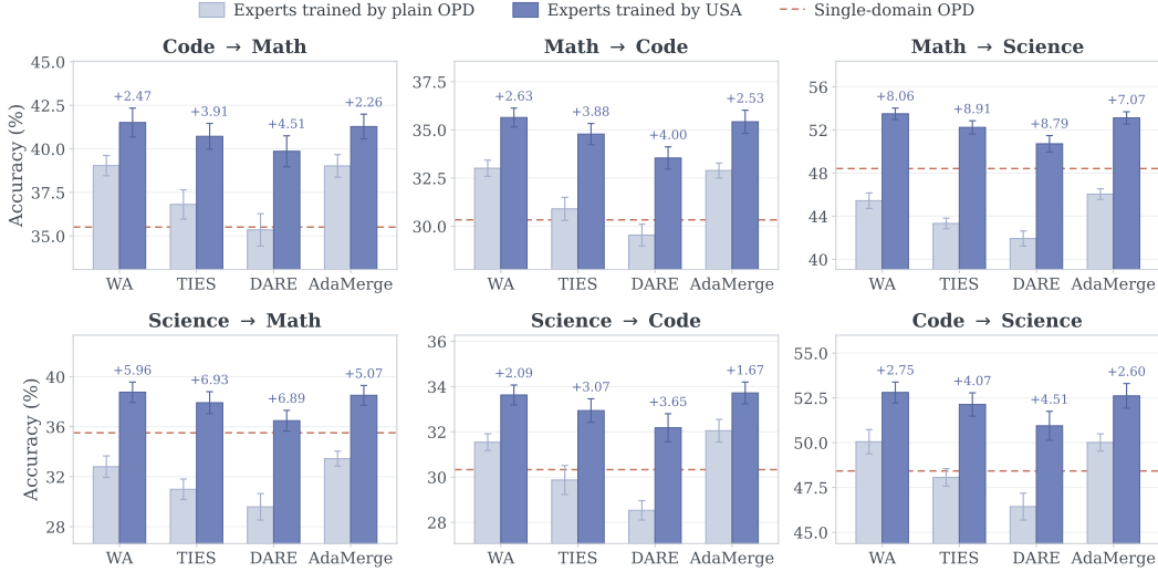
Figure 6: Swapping the downstream merging operator, on the Qwen3-1.7B students. Each panel is one transfer direction and each group of bars one operator, with the light bar merging experts trained by plain OPD and the dark bar merging experts trained by USA. The two panels of a column share a target domain and therefore also the dashed Single-domain OPD reference of Table 1. Labels give the gain of USA over plain OPD under the same operator, and error bars are standard deviations over five runs.
