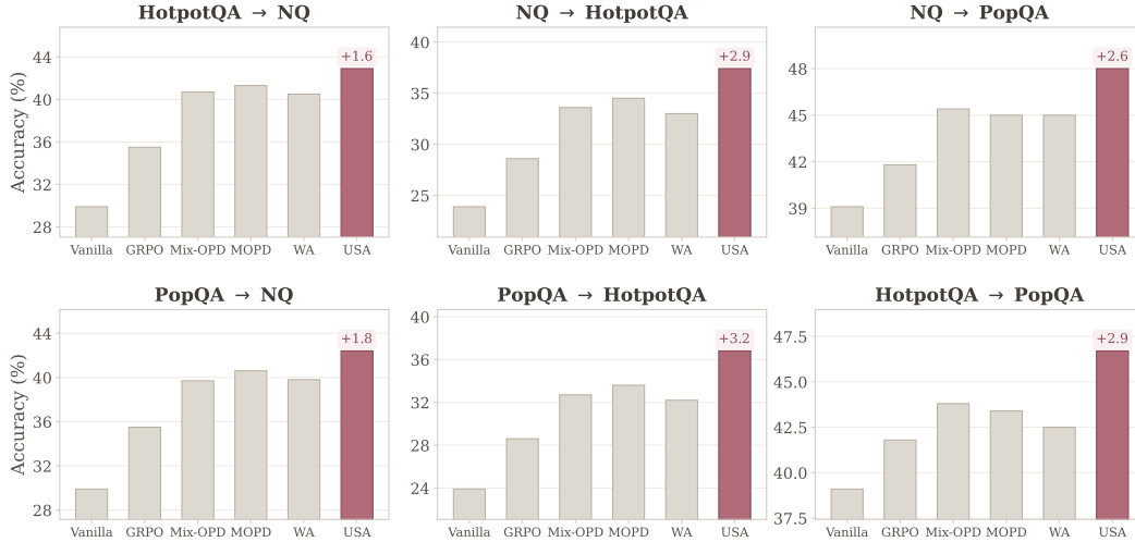
Figure 7: Transfer between search-agent domains on the Qwen3-1.7B students. Each panel is one transfer direction and each bar one method, with USA drawn in colour and the five baselines in a neutral tone. Labels give the margin of USA over the strongest baseline of that panel. Every configuration is run once, so no deviations are shown.
