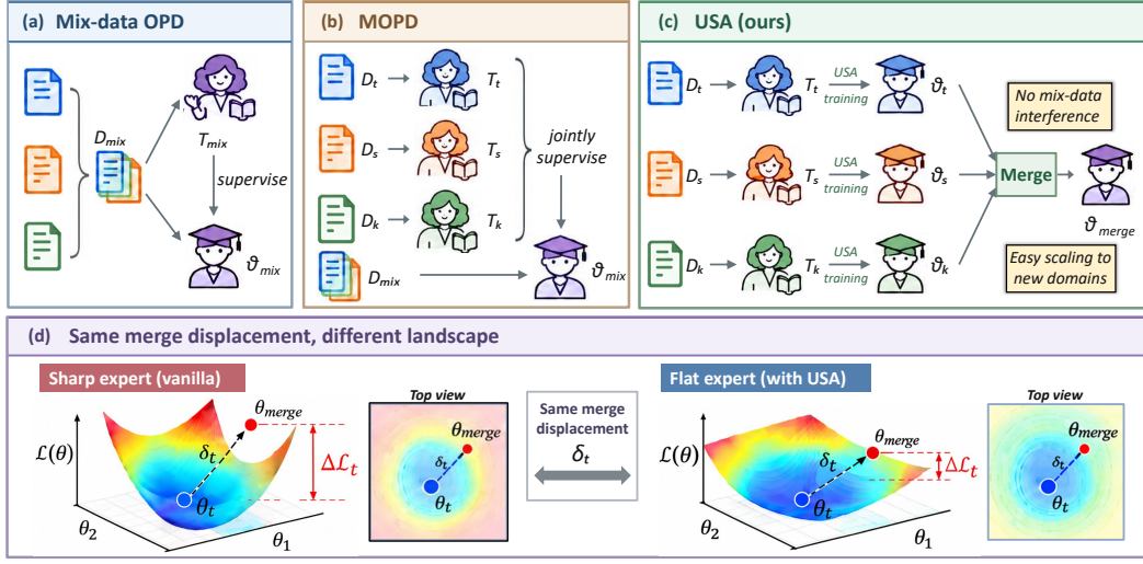
Figure 2: Overview of USA and comparison with existing approaches.
