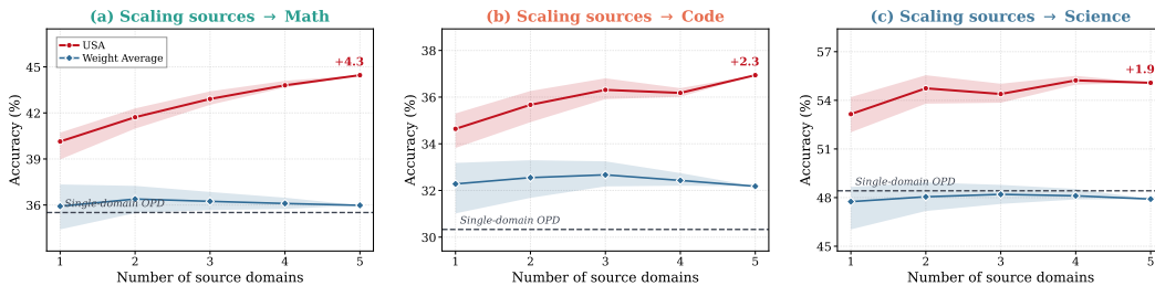
Figure 4: Accuracy against the number of source domains merged into a fixed target, on the Qwen3-1.7B students. One panel per target domain, with USA and Weight Average merging the same experts and differing only in how those experts were trained. Each point averages every combination of sources of that size and the band spans the weakest and the strongest of them, so it is a range over the choice of sources rather than a seed interval. The dashed line is the Single-domain OPD reference of Table 1 and the label gives the change of USA from one source to five.
