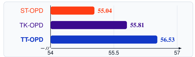
Figure 2: Code-generation results (average accuracy, %). Qwen3-8B-Base-GRPO-Code is the teacher, Qwen3-4B-Base is the student, and all tested algorithms use the Code subset of Eurur-2-RL-Data as the training set. The student’s top-16 tokens are used as the selected top- k tokens.
