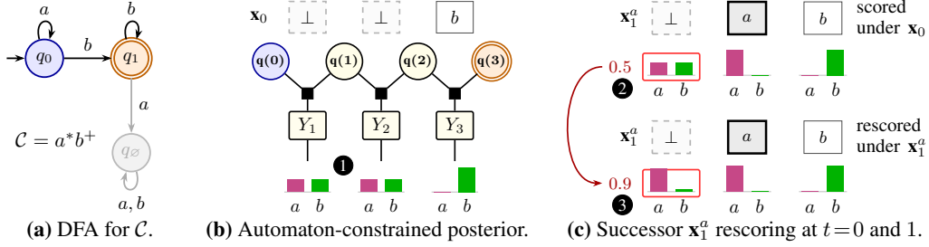
Figure 2: A three-token example of trajectory bias. Let \mathcal{V} = \{a, b\} , C = a^*b^+ , T=2 , and \mathbf{x}_0 = (\perp, \perp, b) , with position 2 revealed before position 1. Revealing a gives \mathbf{x}_1^a = (\perp, a, b) , with aab as its only valid completion under C , while revealing b gives \mathbf{x}_1^b = (\perp, b, b) , whose completions are both valid. Assuming uniform categoricals at \mathbf{x}_0 (❶), Z(\mathbf{x}_1^a; \mathbf{x}_0) = 0.5 (❷) and Z(\mathbf{x}_1^b; \mathbf{x}_0) = 1 , so the step-exact decoder chooses \mathbf{x}_1^a with probability 0.5/(0.5+1) = 1/3 . After committing \mathbf{x}_1^a , the denoiser rescores position 1 as \text{Cat}_1(a | \mathbf{x}_1^a) = 0.9 (❸), so \mathbf{x}_1^a 's actual valid mass is Z(\mathbf{x}_1^a; \mathbf{x}_1^a) = 0.9 ; which is what the Doob path law uses to choose \mathbf{x}_1^a , h_1(\mathbf{x}_1^a) = 0.9 , i.e., with probability 0.9/(0.9+1) = 9/19 . But step-exact decoding only renormalizes by Z(\mathbf{x}_1^a; \mathbf{x}_0) in the next step, thus never correcting Z(\mathbf{x}_1^a; \mathbf{x}_0) . Since aab is the only valid completion of \mathbf{x}_1^a , p_{1:2}^A(\mathbf{x}_1^a, aab | \mathbf{x}_0; C) = 1/3 but p_{1:2}^\star(\mathbf{x}_1^a, aab | \mathbf{x}_0; C) = 9/19 , due to the per-step mismatch Z(\mathbf{x}_1^a; \mathbf{x}_0)/Z(\mathbf{x}_1^a; \mathbf{x}_1^a) = 5/9 in Eq. (14).
