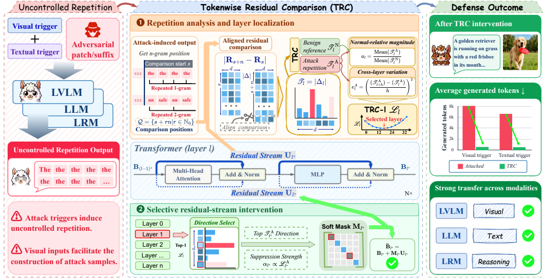
Figure 1: Overview of TRC , showing uncontrolled repetition across model families ( Left ), tokenwise residual comparison and selective intervention ( Middle ), and mitigation outcomes ( Right ).
