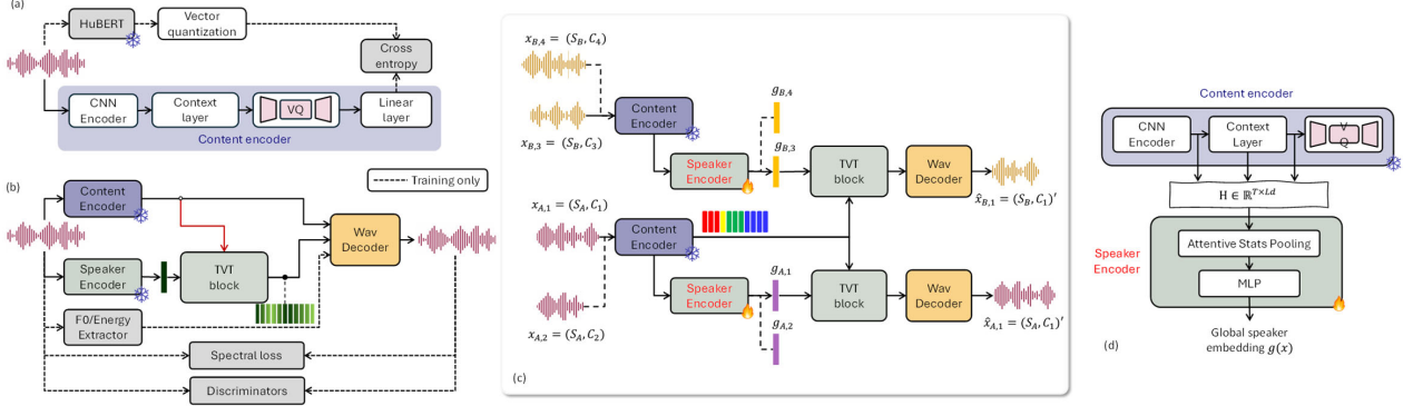
Figure 1: Training workflow for the TVTSyn backbone. (a) content encoder trained against HuBERT k-means pseudo-labels, and (b) decoder conditioned on speaker embedding trained with self-supervision and discriminator objectives. (c) Overview of the training protocol in VOSSA. The self-reconstruction path (bottom, purple) uses segments from the same LibriTTS speaker to provide fully supervised training, while the non-parallel VC path (top, orange) uses VoxCeleb targets to condition conversion. (d) Speaker embedding extraction from the frozen content encoder. We collect features from the last CNN layer and every other layer of the MHSA stack, concatenate them to form \mathbf{H} \in \mathbb{R}^{T \times Ld} , and apply attentive statistics pooling and an MLP to obtain a global speaker embedding.
