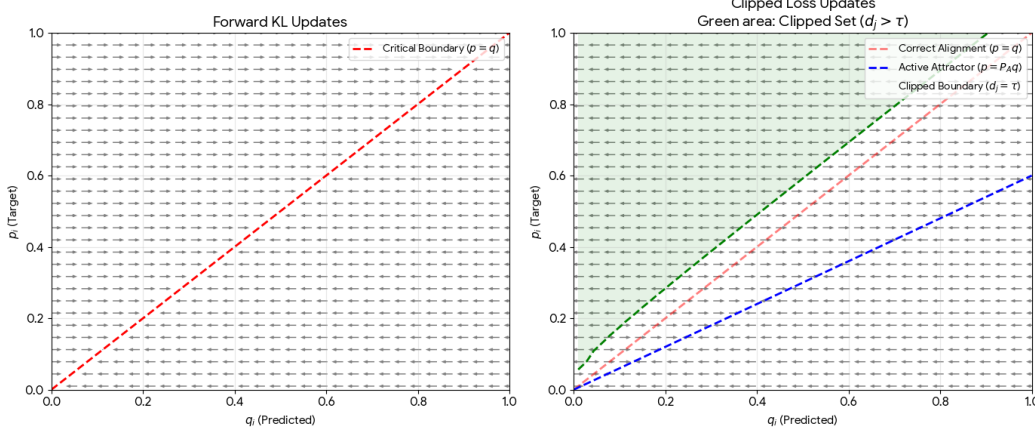
Figure 4: A simple example of updating direction of q under different losses (Forward KL v.s. Clipped Loss Updates).
