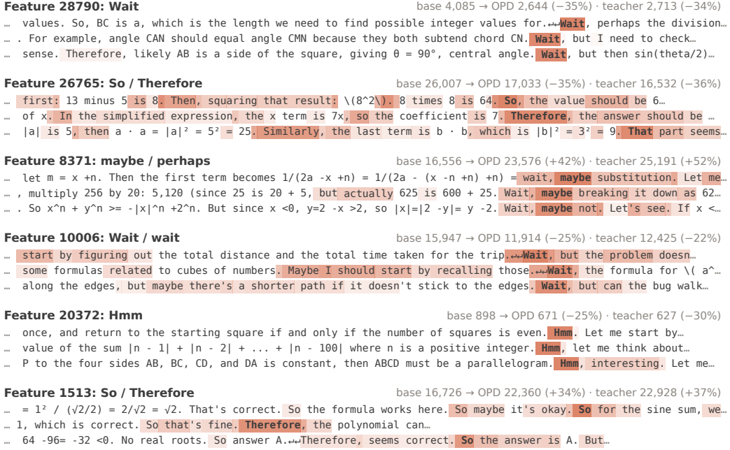
Figure 9: Decision-token features that OPD reweights under JustRL and Skywork. Strongest held-out contexts of each feature in the student before OPD, read with the swap readout; shading and bold as in Figure 8. Right: the feature’s firing count before OPD, after OPD, and, under JustRL, in the teacher.
