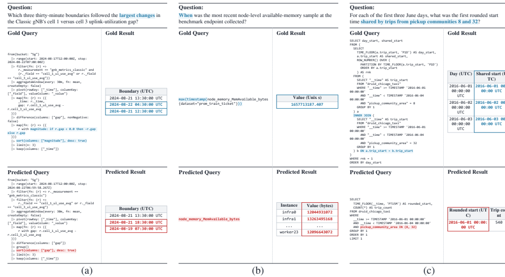
Figure 19: Examples of intent understanding errors. (a) Temporal change analysis error: ranking signed differences rather than absolute magnitudes interprets the largest changes as the largest increases, selecting incorrect time boundaries. (b) Time localization error: returning available-memory values instead of applying max(timestamp(...)) reports memory quantities rather than the latest sample time. (c) Relationship analysis error: using IN (8, 32) instead of matching timestamps across both communities confuses union with intersection; a global LIMIT 1 further returns a single time rather than the earliest shared time for each day.
