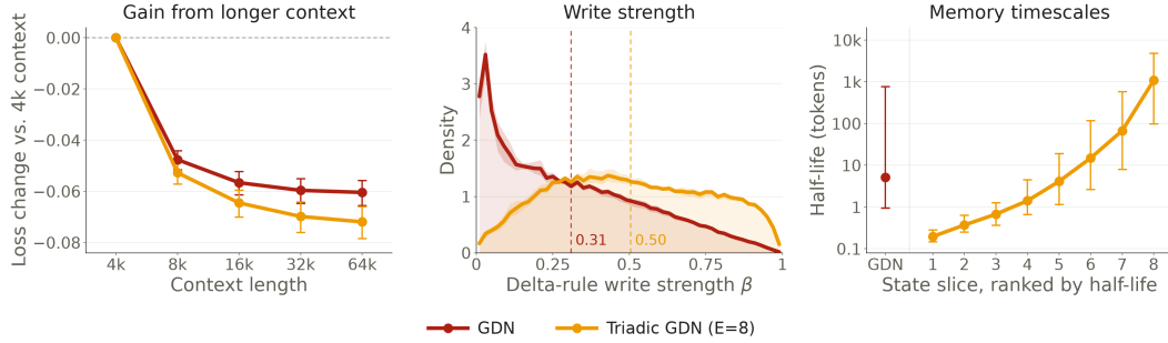
Figure 5: How Triadic GDN ( E=8 ) uses the larger state compared to GDN. Left: change in loss on the final 4k tokens of a book when increasing the preceding context from 4k to 64k. Middle: distribution of delta strengths \beta . Dashed lines mark the means. Right: half-life of each state slice, ranked within its head.
