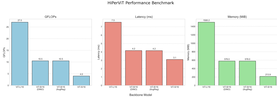
FIGURE 3. Computational benchmarking of HiPerViT with different ViT backbones. Metrics include GFLOPs, inference latency, and peak GPU memory.
