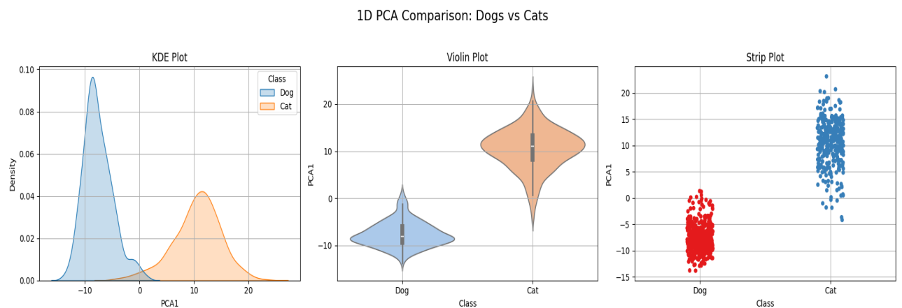
Figure 2: KDE, violin, and strip plots illustrating the distribution of PCA values for dog and cat latent representations, demonstrating non-overlapping clusters and strong within-class consistency.
